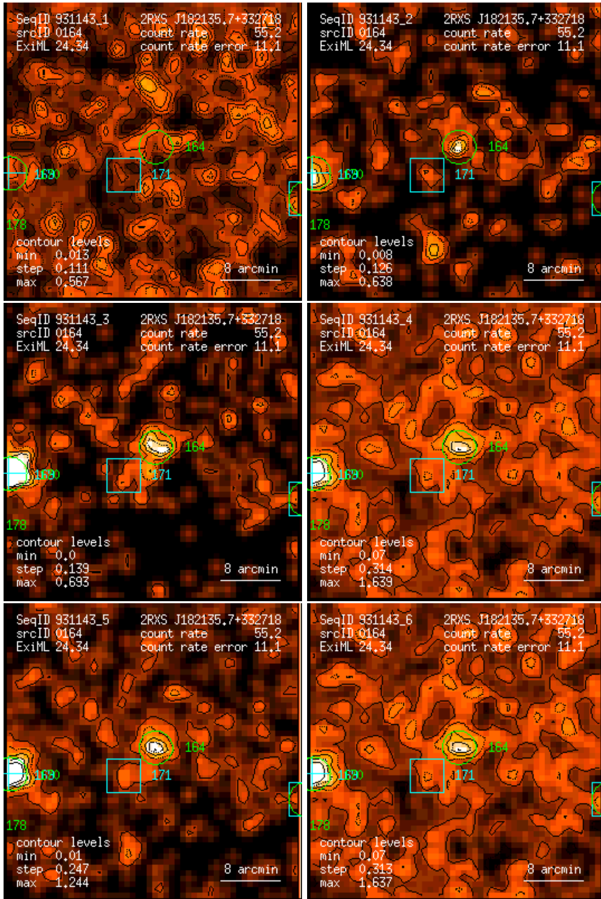
Figure 164: RASS 931143: detection 0164: band rate images, Gaussian filter: (1) PSPC channels 11 – 41, (2) 52 – 90, (3) 91 – 201, (4) 11 – 235, (5) 52 – 201, (6) 11 – 201. Broad band rates in counts/ks. Band rate contour levels in counts/ks/arcmin 2 .
