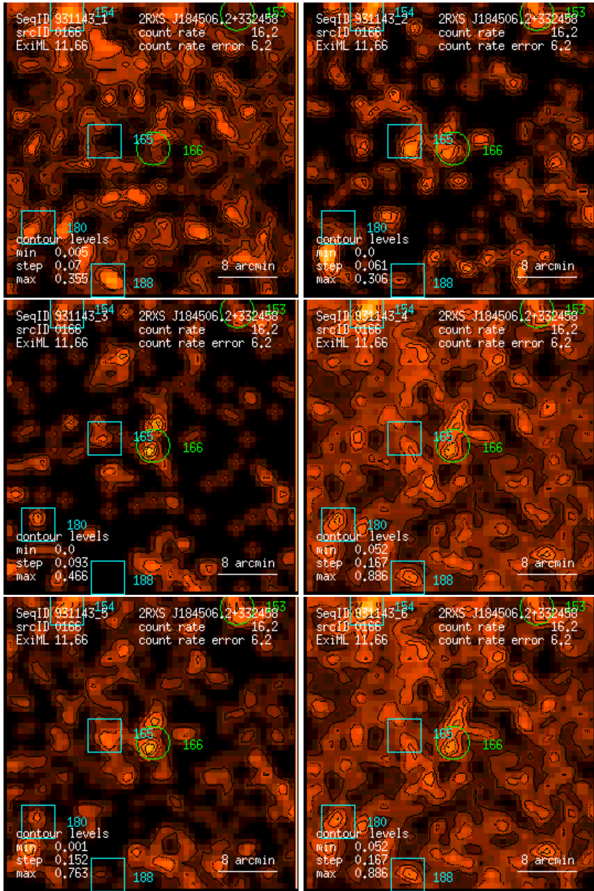
Figure 166: RASS 931143: detection 0166: band rate images, Gaussian filter: (1) PSPC channels 11 – 41, (2) 52 – 90, (3) 91 – 201, (4) 11 – 235, (5) 52 – 201, (6) 11 – 201. Broad band rates in counts/ks. Band rate contour levels in counts/ks/arcmin 2 .
