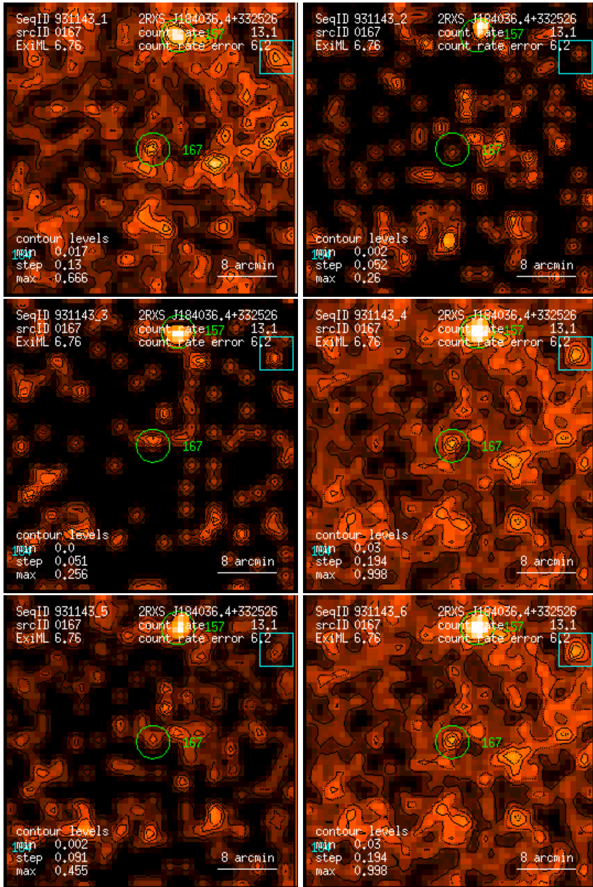
Figure 167: RASS 931143: detection 0167: band rate images, Gaussian filter: (1) PSPC channels 11 – 41, (2) 52 – 90, (3) 91 – 201, (4) 11 – 235, (5) 52 – 201, (6) 11 – 201. Broad band rates in counts/ks. Band rate contour levels in counts/ks/arcmin 2 .
