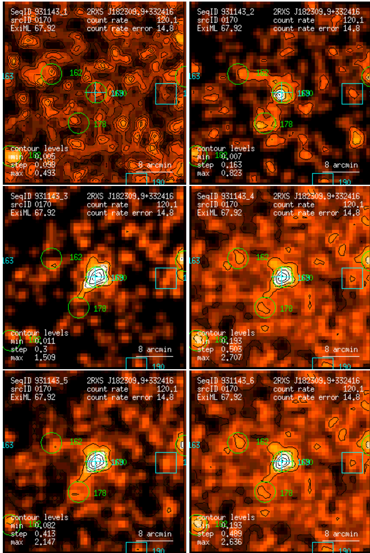
Figure 170: RASS 931143: detection 0170: band rate images, Gaussian filter: (1) PSPC channels 11 – 41, (2) 52 – 90, (3) 91 – 201, (4) 11 – 235, (5) 52 – 201, (6) 11 – 201. Broad band rates in counts/ks. Band rate contour levels in counts/ks/arcmin 2 .
