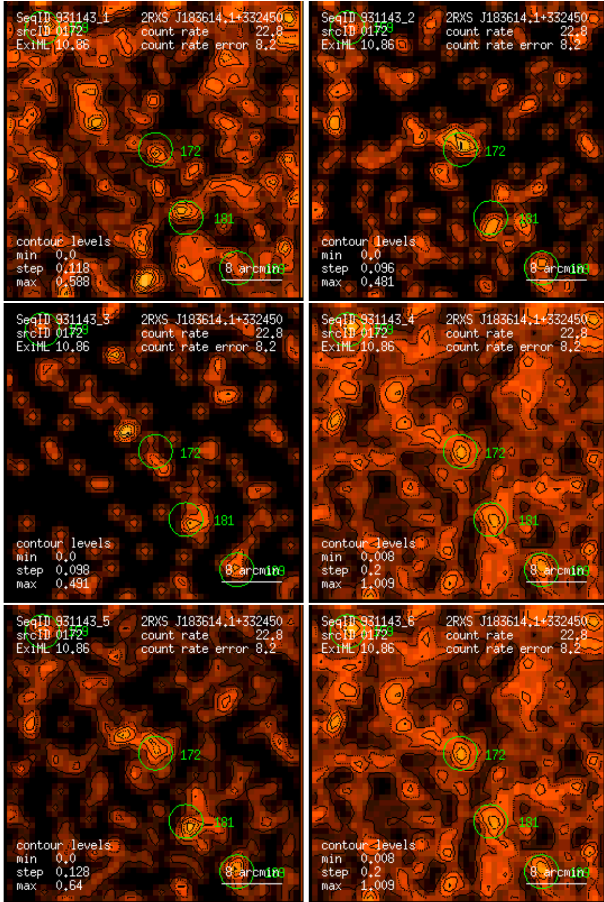
Figure 172: RASS 931143: detection 0172: band rate images, Gaussian filter: (1) PSPC channels 11 – 41, (2) 52 – 90, (3) 91 – 201, (4) 11 – 235, (5) 52 – 201, (6) 11 – 201. Broad band rates in counts/ks. Band rate contour levels in counts/ks/arcmin 2 .
