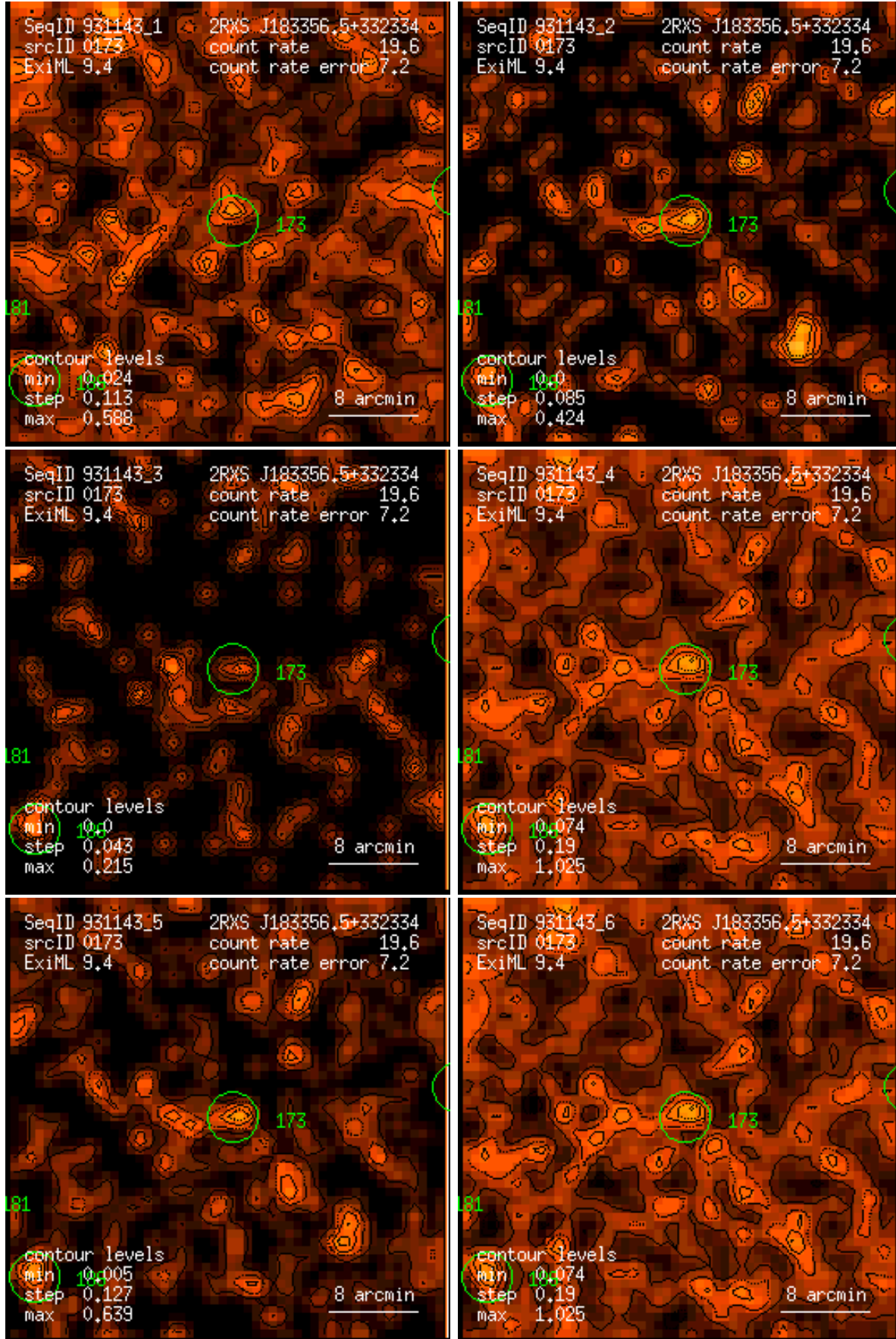
Figure 173: RASS 931143: detection 0173: band rate images, Gaussian filter: (1) PSPC channels 11 – 41, (2) 52 – 90, (3) 91 – 201, (4) 11 – 235, (5) 52 – 201, (6) 11 – 201. Broad band rates in counts/ks. Band rate contour levels in counts/ks/arcmin 2 .
