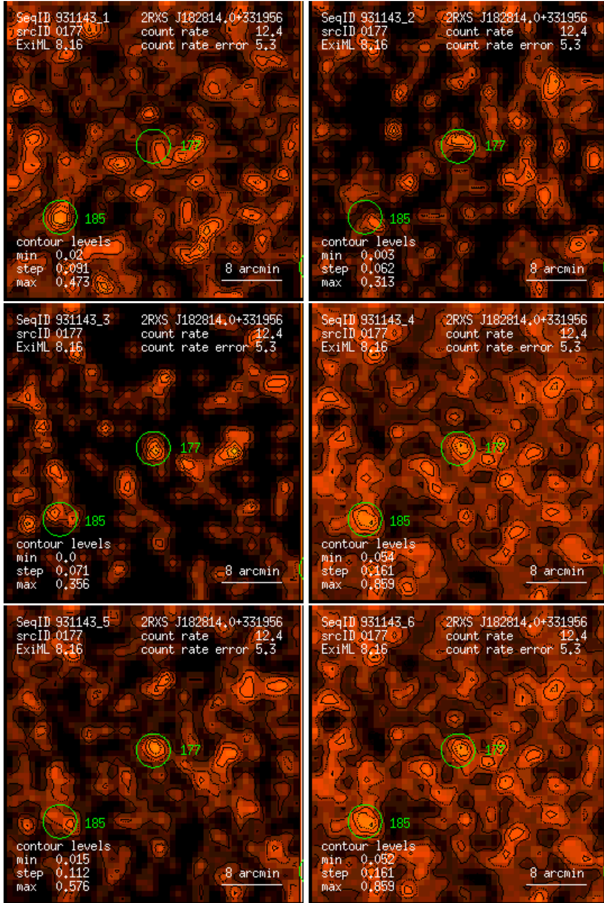
Figure 177: RASS 931143: detection 0177: band rate images, Gaussian filter: (1) PSPC channels 11 – 41, (2) 52 – 90, (3) 91 – 201, (4) 11 – 235, (5) 52 – 201, (6) 11 – 201. Broad band rates in counts/ks. Band rate contour levels in counts/ks/arcmin 2 .
