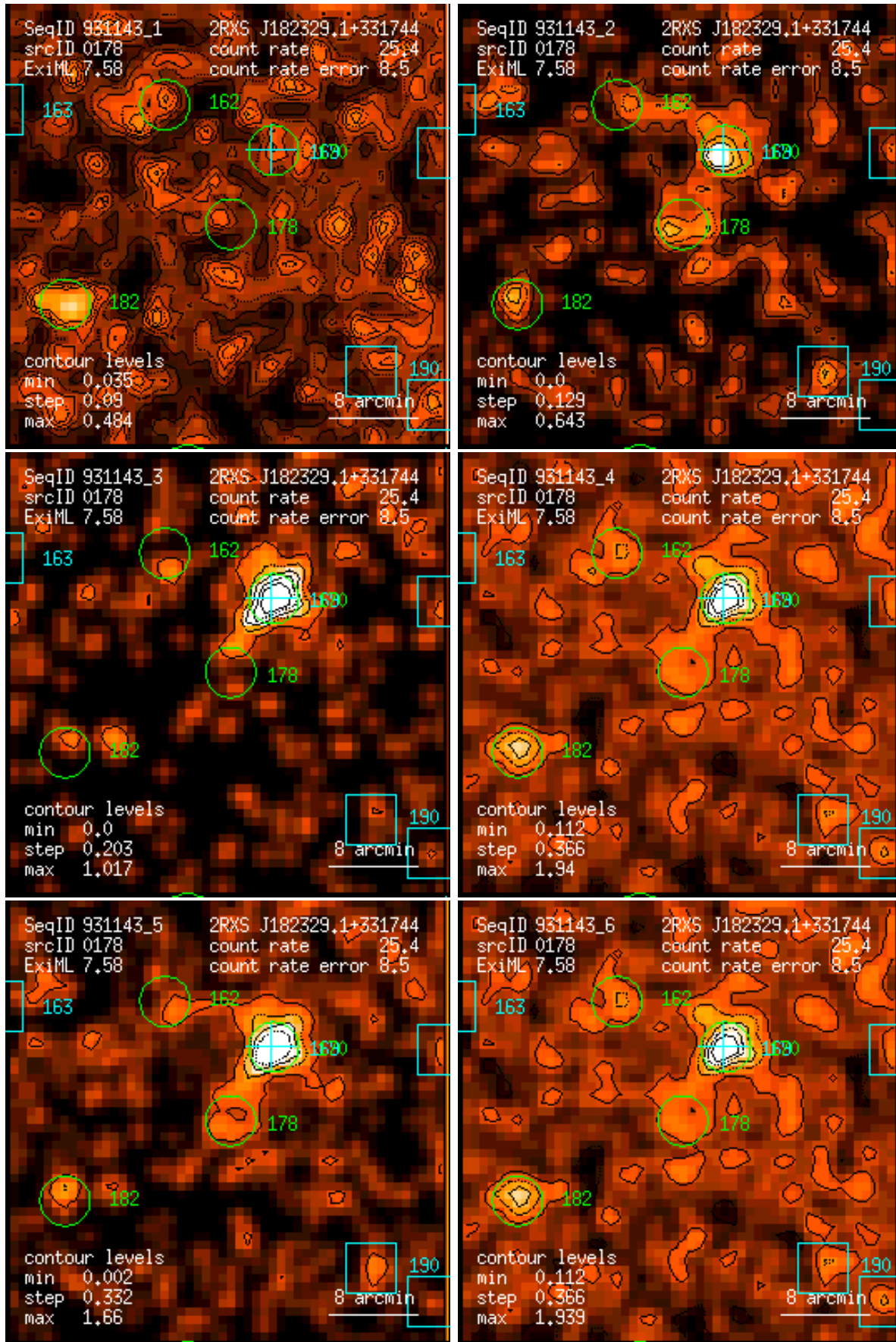
Figure 178: RASS 931143: detection 0178: band rate images, Gaussian filter: (1) PSPC channels 11 – 41, (2) 52 – 90, (3) 91 – 201, (4) 11 – 235, (5) 52 – 201, (6) 11 – 201. Broad band rates in counts/ks. Band rate contour levels in counts/ks/arcmin 2 .
