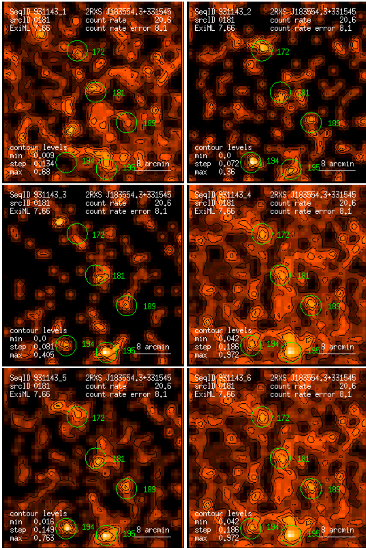
Figure 181: RASS 931143: detection 0181: band rate images, Gaussian filter: (1) PSPC channels 11 – 41, (2) 52 – 90, (3) 91 – 201, (4) 11 – 235, (5) 52 – 201, (6) 11 – 201. Broad band rates in counts/ks. Band rate contour levels in counts/ks/arcmin 2 .
