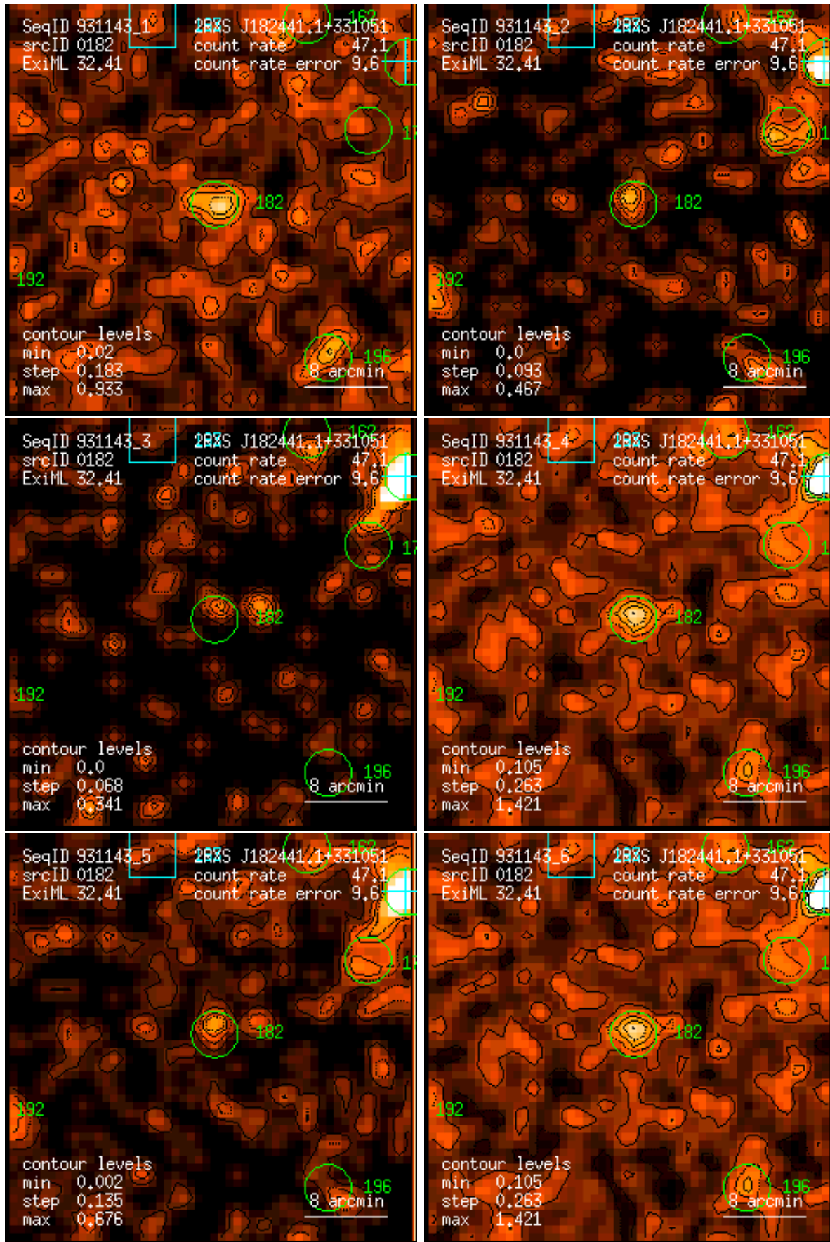
Figure 182: RASS 931143: detection 0182: band rate images, Gaussian filter: (1) PSPC channels 11 – 41, (2) 52 – 90, (3) 91 – 201, (4) 11 – 235, (5) 52 – 201, (6) 11 – 201. Broad band rates in counts/ks. Band rate contour levels in counts/ks/arcmin 2 .
