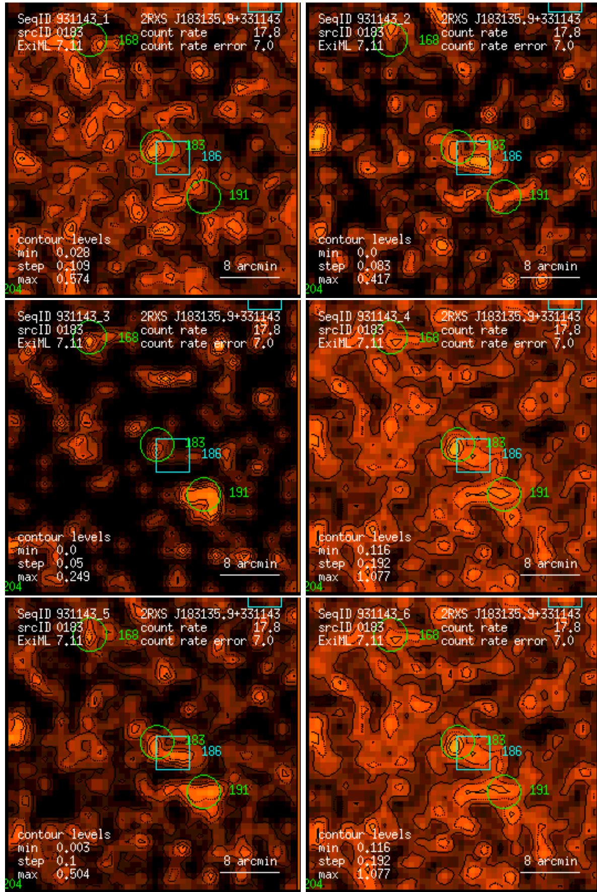
Figure 183: RASS 931143: detection 0183: band rate images, Gaussian filter: (1) PSPC channels 11 – 41, (2) 52 – 90, (3) 91 – 201, (4) 11 – 235, (5) 52 – 201, (6) 11 – 201. Broad band rates in counts/ks. Band rate contour levels in counts/ks/arcmin 2 .
