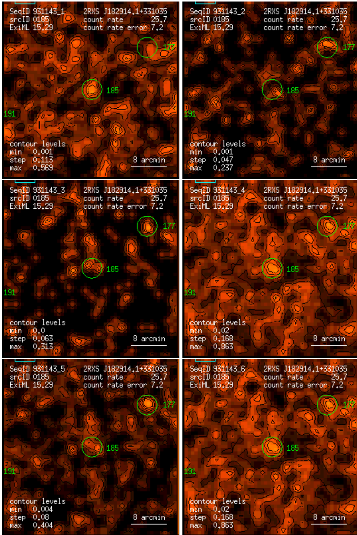
Figure 185: RASS 931143: detection 0185: band rate images, Gaussian filter: (1) PSPC channels 11 – 41, (2) 52 – 90, (3) 91 – 201, (4) 11 – 235, (5) 52 – 201, (6) 11 – 201. Broad band rates in counts/ks. Band rate contour levels in counts/ks/arcmin 2 .
