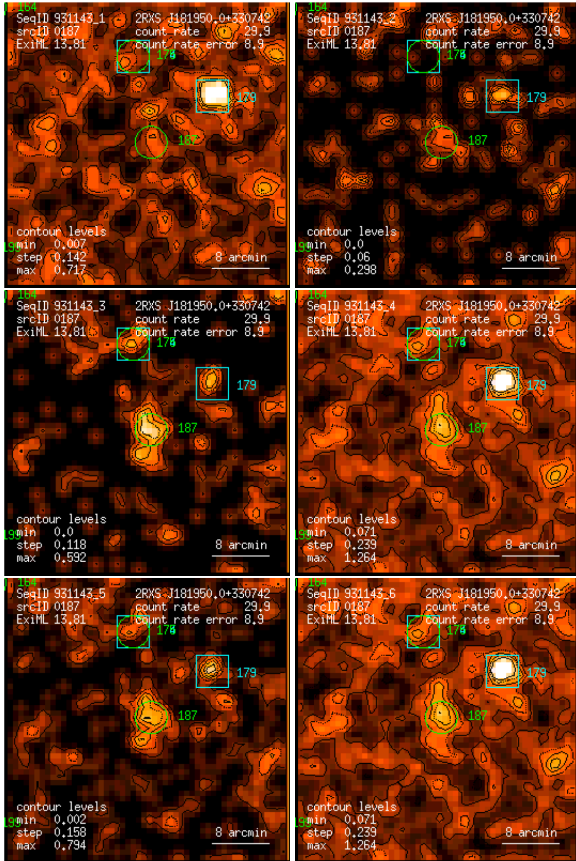
Figure 187: RASS 931143: detection 0187: band rate images, Gaussian filter: (1) PSPC channels 11 – 41, (2) 52 – 90, (3) 91 – 201, (4) 11 – 235, (5) 52 – 201, (6) 11 – 201. Broad band rates in counts/ks. Band rate contour levels in counts/ks/arcmin 2 .
