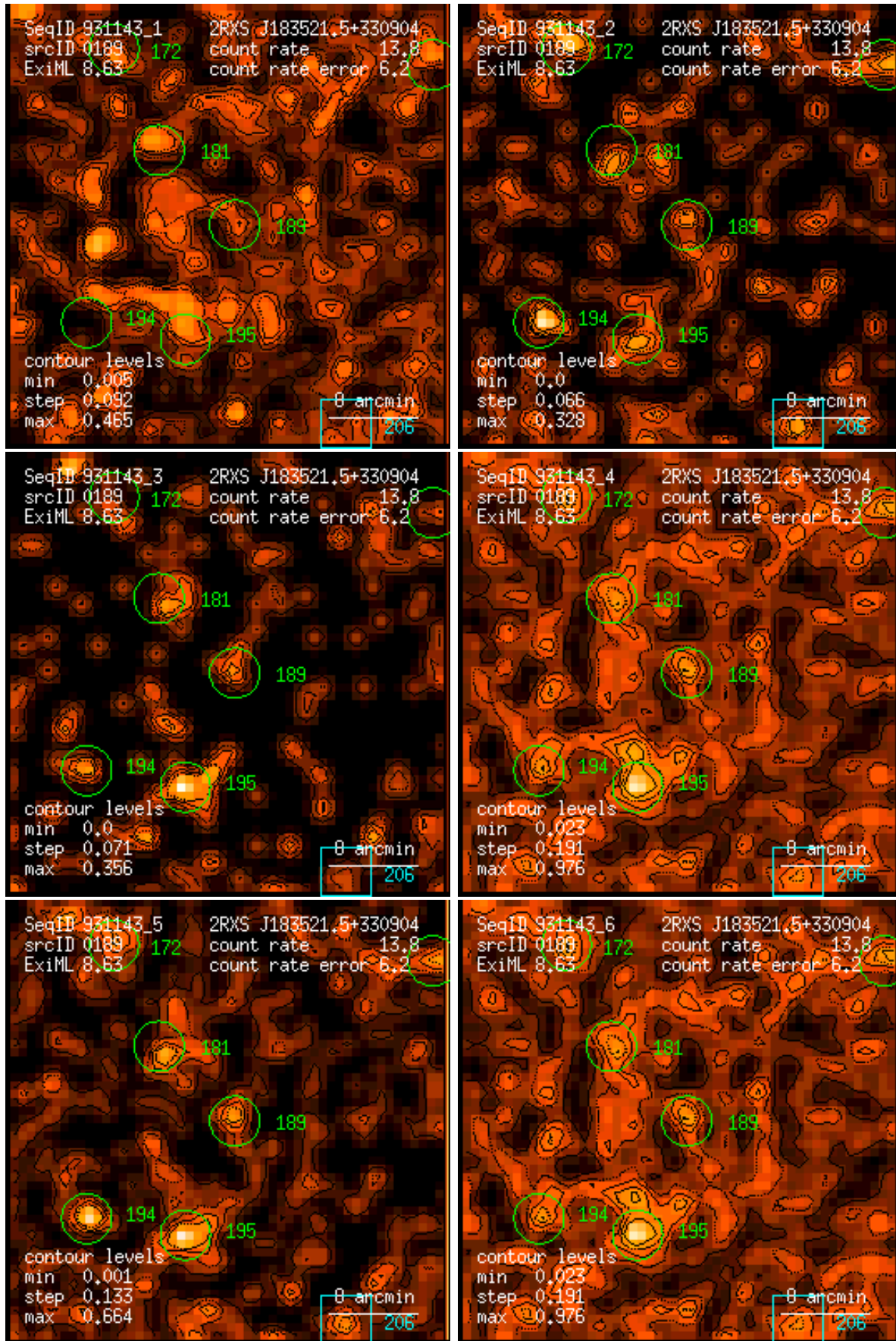
Figure 189: RASS 931143: detection 0189: band rate images, Gaussian filter: (1) PSPC channels 11 – 41, (2) 52 – 90, (3) 91 – 201, (4) 11 – 235, (5) 52 – 201, (6) 11 – 201. Broad band rates in counts/ks. Band rate contour levels in counts/ks/arcmin 2 .
