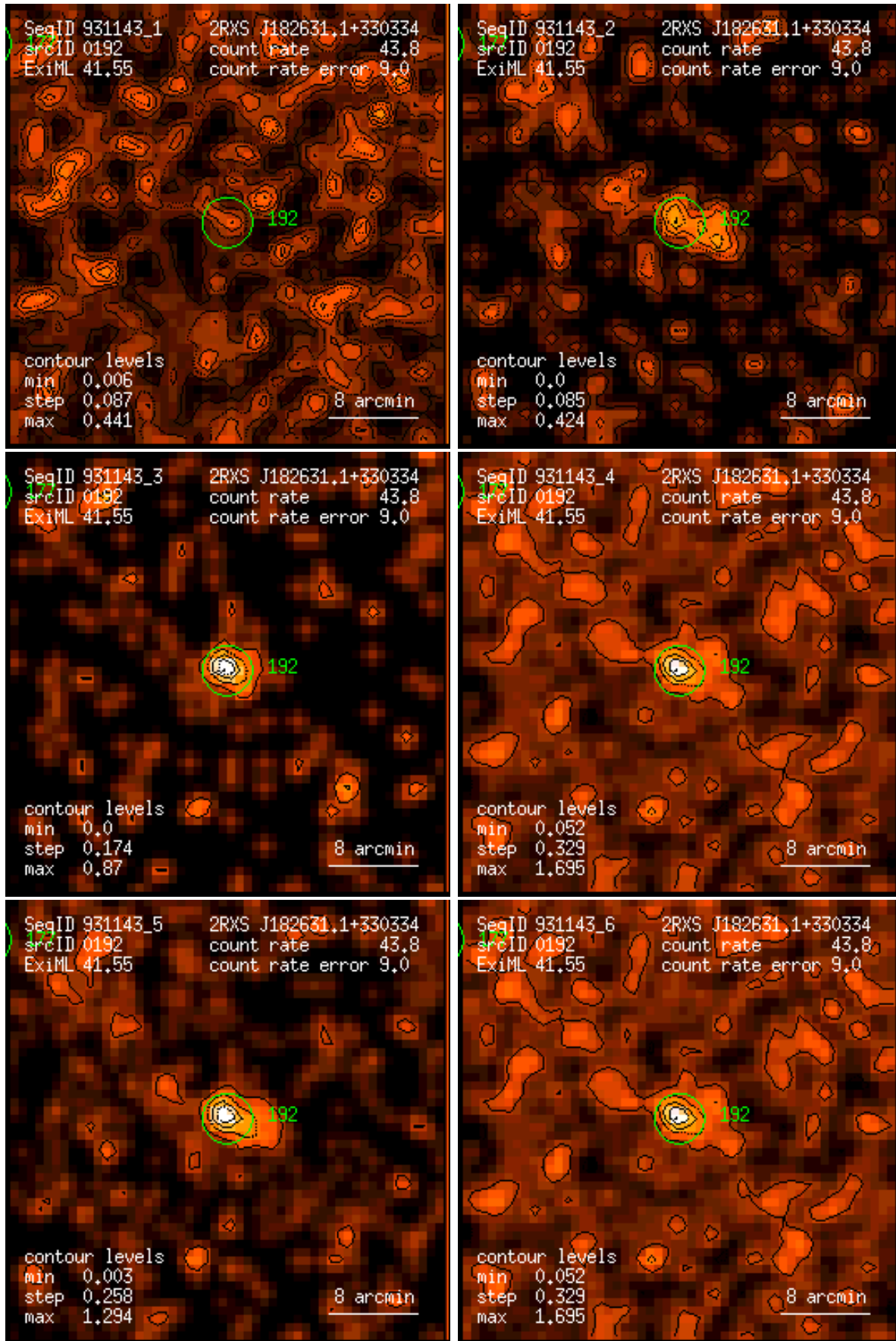
Figure 192: RASS 931143: detection 0192: band rate images, Gaussian filter: (1) PSPC channels 11 – 41, (2) 52 – 90, (3) 91 – 201, (4) 11 – 235, (5) 52 – 201, (6) 11 – 201. Broad band rates in counts/ks. Band rate contour levels in counts/ks/arcmin 2 .
