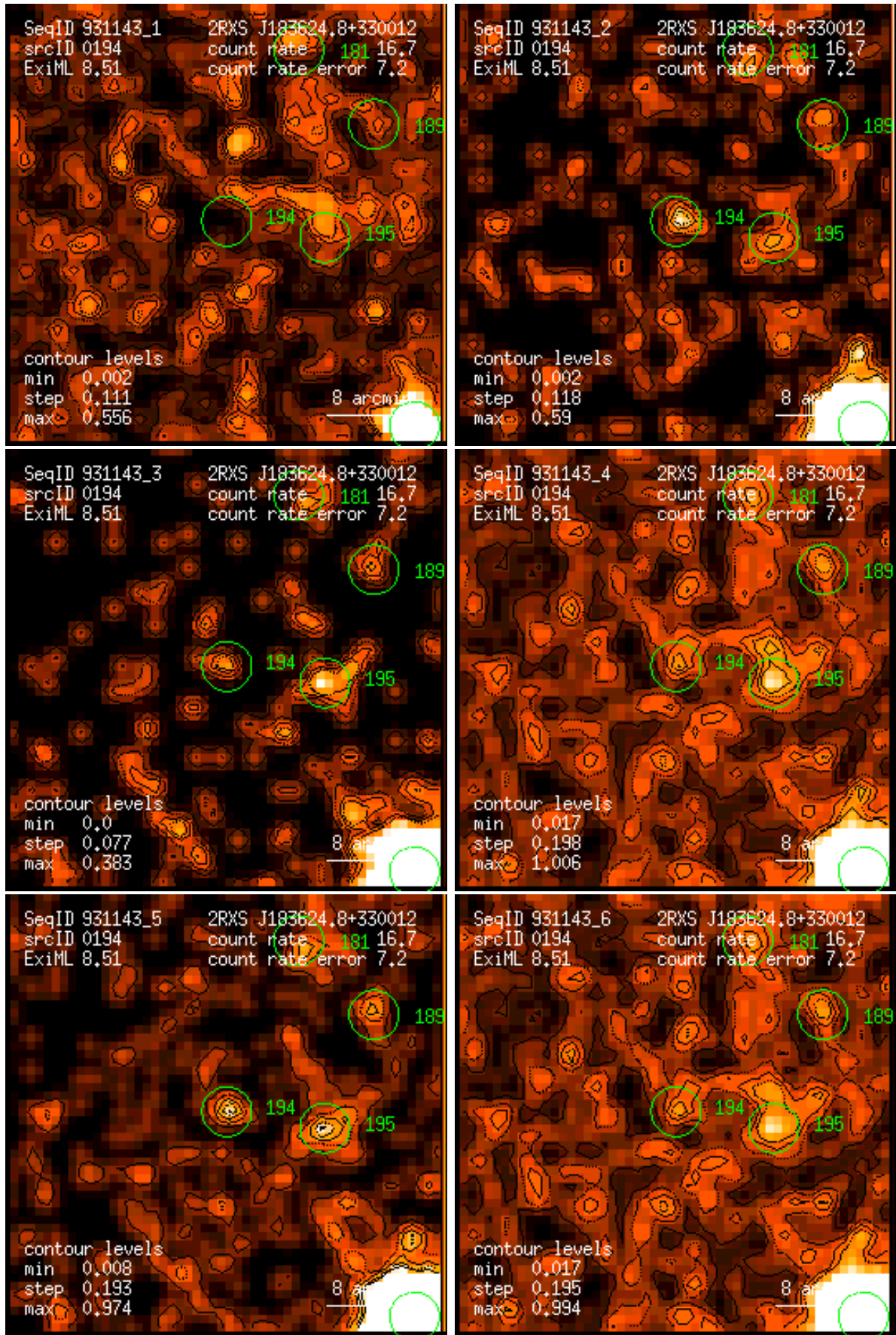
Figure 194: RASS 931143: detection 0194: band rate images, Gaussian filter: (1) PSPC channels 11 – 41, (2) 52 – 90, (3) 91 – 201, (4) 11 – 235, (5) 52 – 201, (6) 11 – 201. Broad band rates in counts/ks. Band rate contour levels in counts/ks/arcmin 2 .
