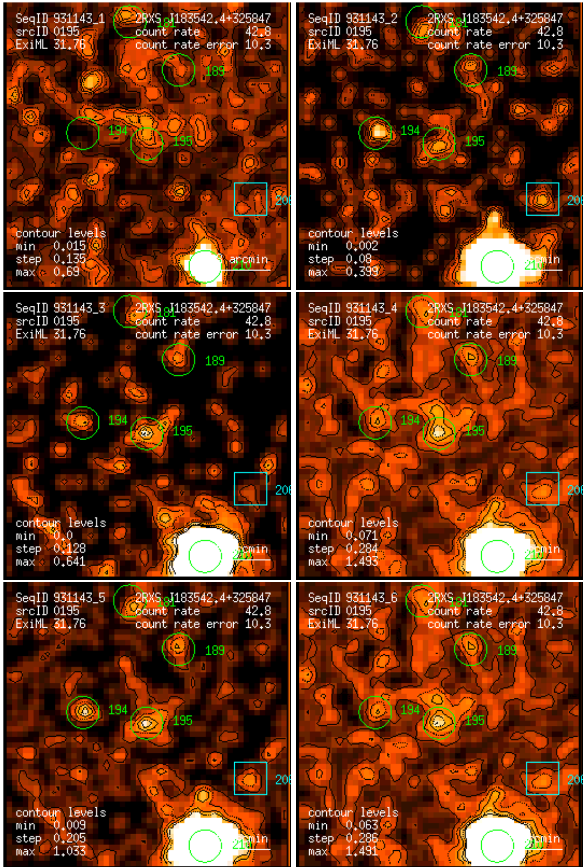
Figure 195: RASS 931143: detection 0195: band rate images, Gaussian filter: (1) PSPC channels 11 – 41, (2) 52 – 90, (3) 91 – 201, (4) 11 – 235, (5) 52 – 201, (6) 11 – 201. Broad band rates in counts/ks. Band rate contour levels in counts/ks/arcmin 2 .
