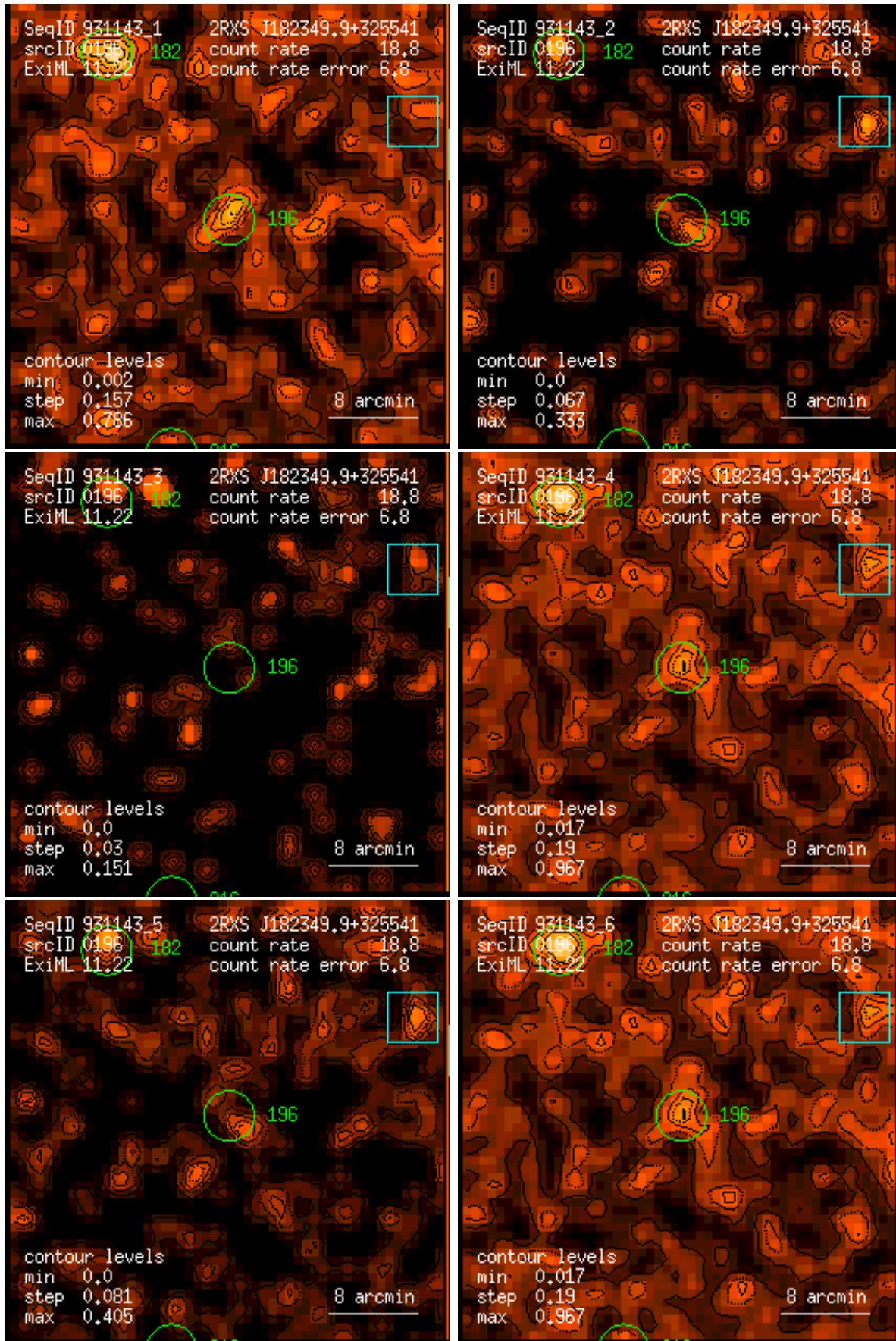
Figure 196: RASS 931143: detection 0196: band rate images, Gaussian filter: (1) PSPC channels 11 – 41, (2) 52 – 90, (3) 91 – 201, (4) 11 – 235, (5) 52 – 201, (6) 11 – 201. Broad band rates in counts/ks. Band rate contour levels in counts/ks/arcmin 2 .
