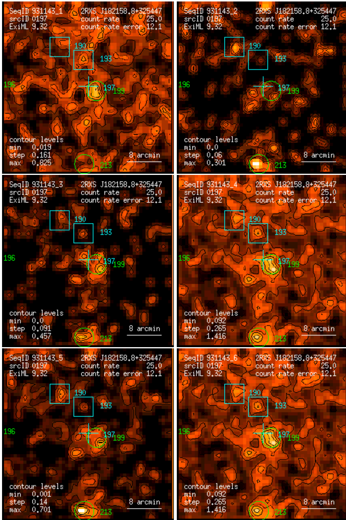
Figure 197: RASS 931143: detection 0197: band rate images, Gaussian filter: (1) PSPC channels 11 – 41, (2) 52 – 90, (3) 91 – 201, (4) 11 – 235, (5) 52 – 201, (6) 11 – 201. Broad band rates in counts/ks. Band rate contour levels in counts/ks/arcmin 2 .
