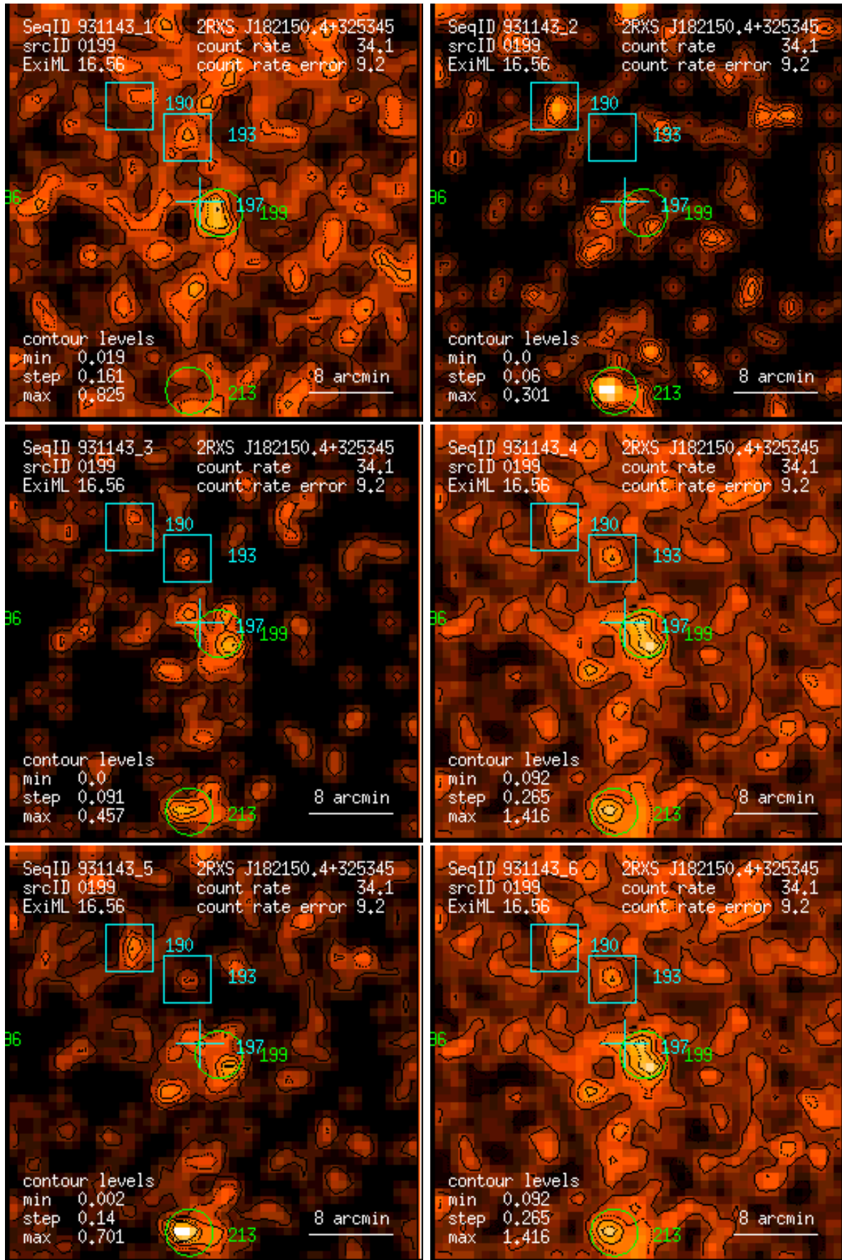
Figure 199: RASS 931143: detection 0199: band rate images, Gaussian filter: (1) PSPC channels 11 – 41, (2) 52 – 90, (3) 91 – 201, (4) 11 – 235, (5) 52 – 201, (6) 11 – 201. Broad band rates in counts/ks. Band rate contour levels in counts/ks/arcmin 2 .
