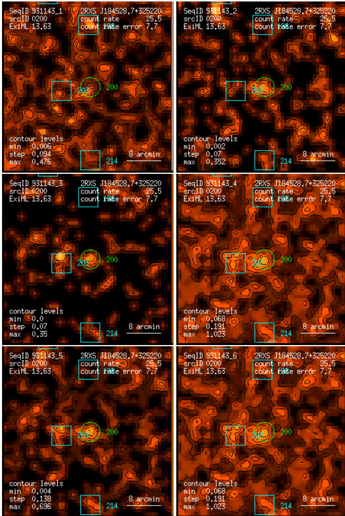
Figure 200: RASS 931143: detection 0200: band rate images, Gaussian filter: (1) PSPC channels 11 – 41, (2) 52 – 90, (3) 91 – 201, (4) 11 – 235, (5) 52 – 201, (6) 11 – 201. Broad band rates in counts/ks. Band rate contour levels in counts/ks/arcmin 2 .
