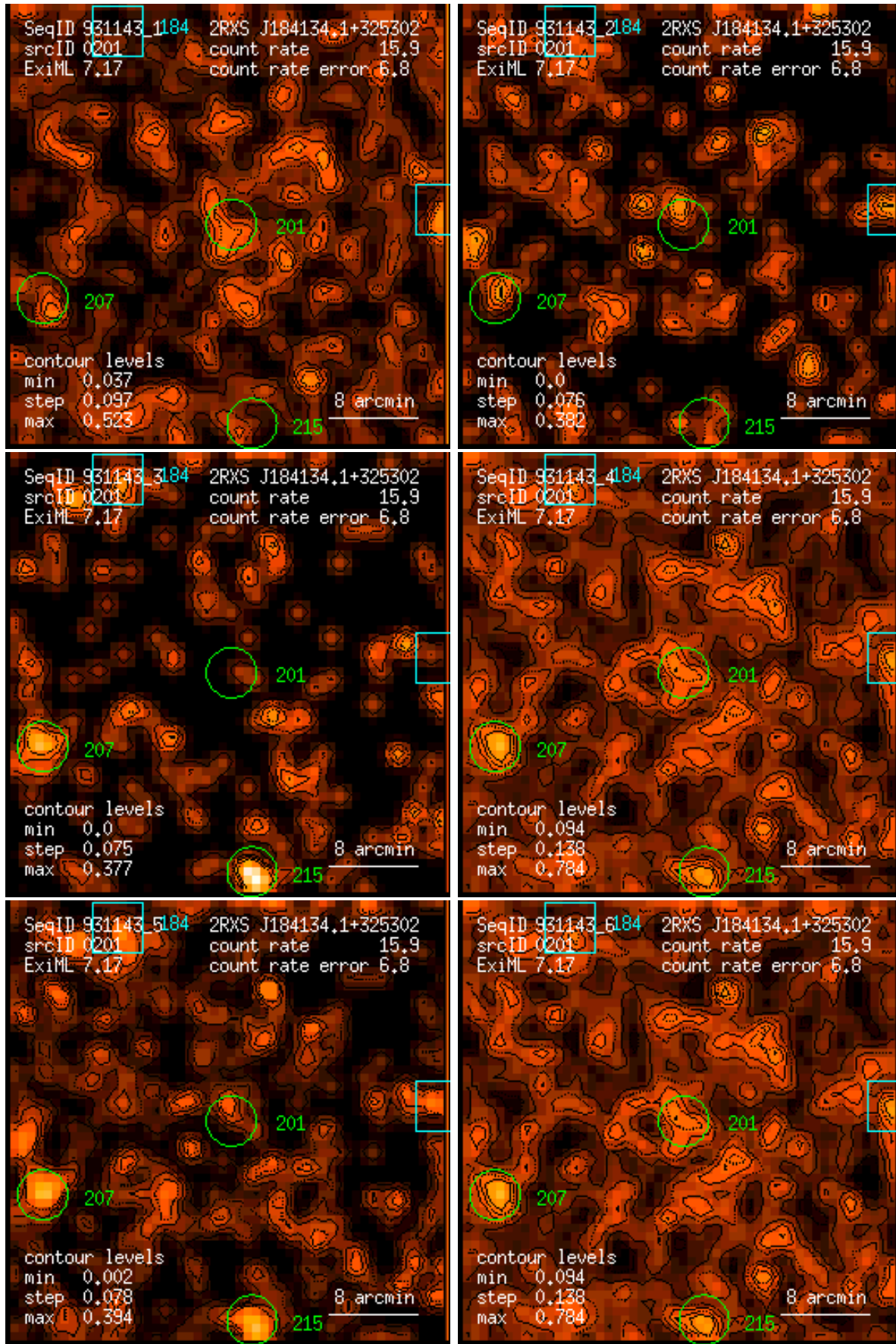
Figure 201: RASS 931143: detection 0201: band rate images, Gaussian filter: (1) PSPC channels 11 – 41, (2) 52 – 90, (3) 91 – 201, (4) 11 – 235, (5) 52 – 201, (6) 11 – 201. Broad band rates in counts/ks. Band rate contour levels in counts/ks/arcmin 2 .
