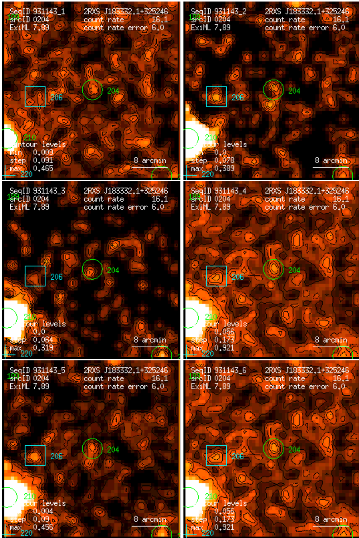
Figure 204: RASS 931143: detection 0204: band rate images, Gaussian filter: (1) PSPC channels 11 – 41, (2) 52 – 90, (3) 91 – 201, (4) 11 – 235, (5) 52 – 201, (6) 11 – 201. Broad band rates in counts/ks. Band rate contour levels in counts/ks/arcmin 2 .
