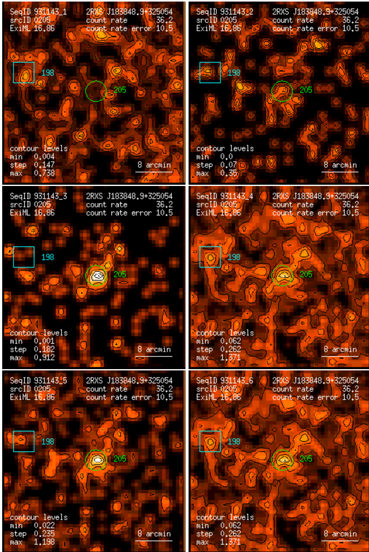
Figure 205: RASS 931143: detection 0205: band rate images, Gaussian filter: (1) PSPC channels 11 – 41, (2) 52 – 90, (3) 91 – 201, (4) 11 – 235, (5) 52 – 201, (6) 11 – 201. Broad band rates in counts/ks. Band rate contour levels in counts/ks/arcmin 2 .
