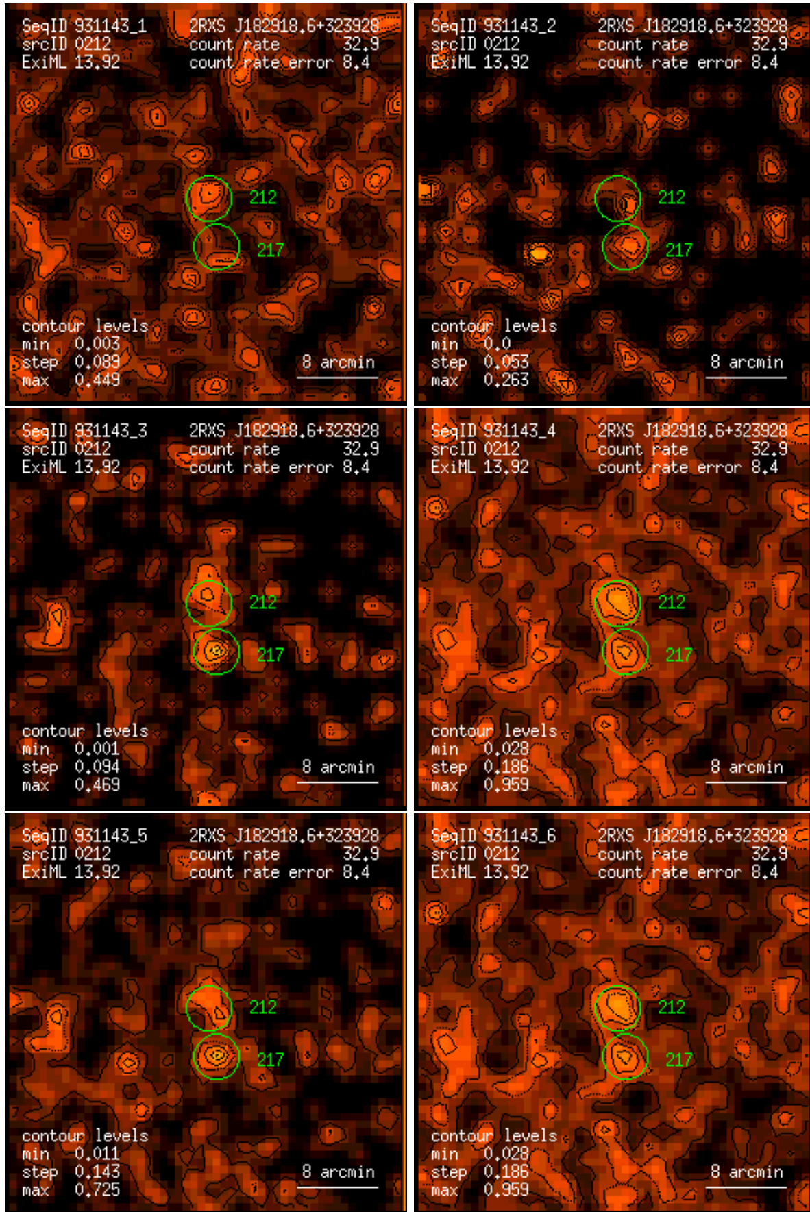
Figure 212: RASS 931143: detection 0212: band rate images, Gaussian filter: (1) PSPC channels 11 – 41, (2) 52 – 90, (3) 91 – 201, (4) 11 – 235, (5) 52 – 201, (6) 11 – 201. Broad band rates in counts/ks. Band rate contour levels in counts/ks/arcmin 2 .
