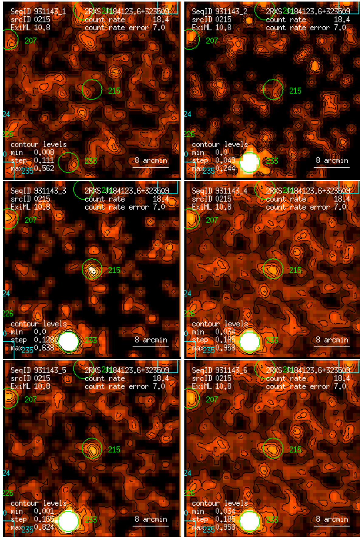
Figure 215: RASS 931143: detection 0215: band rate images, Gaussian filter: (1) PSPC channels 11 – 41, (2) 52 – 90, (3) 91 – 201, (4) 11 – 235, (5) 52 – 201, (6) 11 – 201. Broad band rates in counts/ks. Band rate contour levels in counts/ks/arcmin 2 .
