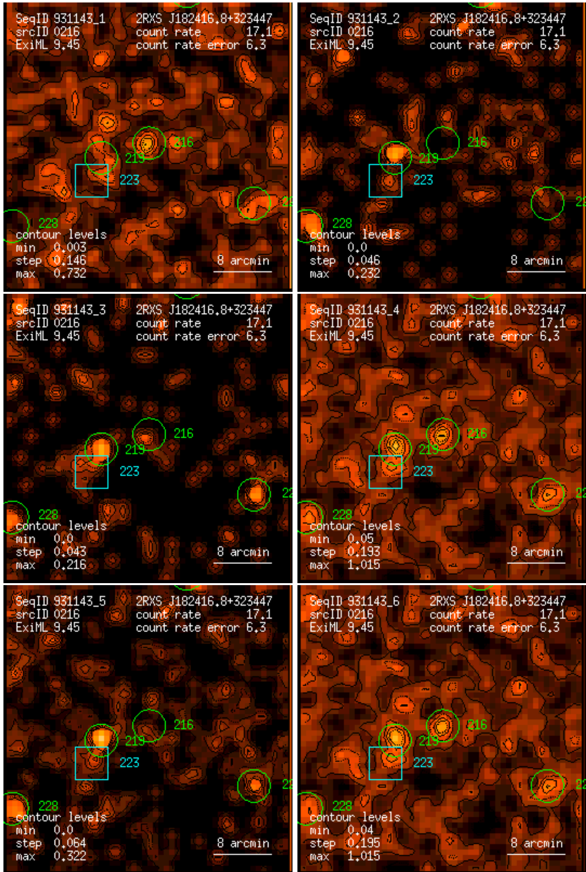
Figure 216: RASS 931143: detection 0216: band rate images, Gaussian filter: (1) PSPC channels 11 – 41, (2) 52 – 90, (3) 91 – 201, (4) 11 – 235, (5) 52 – 201, (6) 11 – 201. Broad band rates in counts/ks. Band rate contour levels in counts/ks/arcmin 2 .
