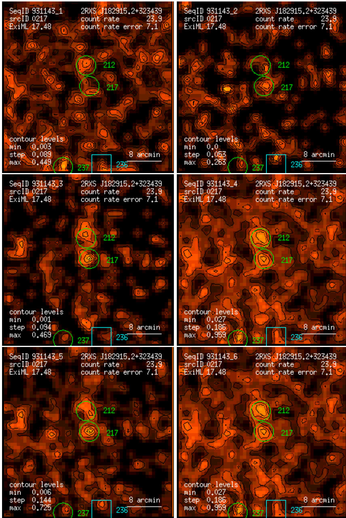
Figure 217: RASS 931143: detection 0217: band rate images, Gaussian filter: (1) PSPC channels 11 – 41, (2) 52 – 90, (3) 91 – 201, (4) 11 – 235, (5) 52 – 201, (6) 11 – 201. Broad band rates in counts/ks. Band rate contour levels in counts/ks/arcmin 2 .
