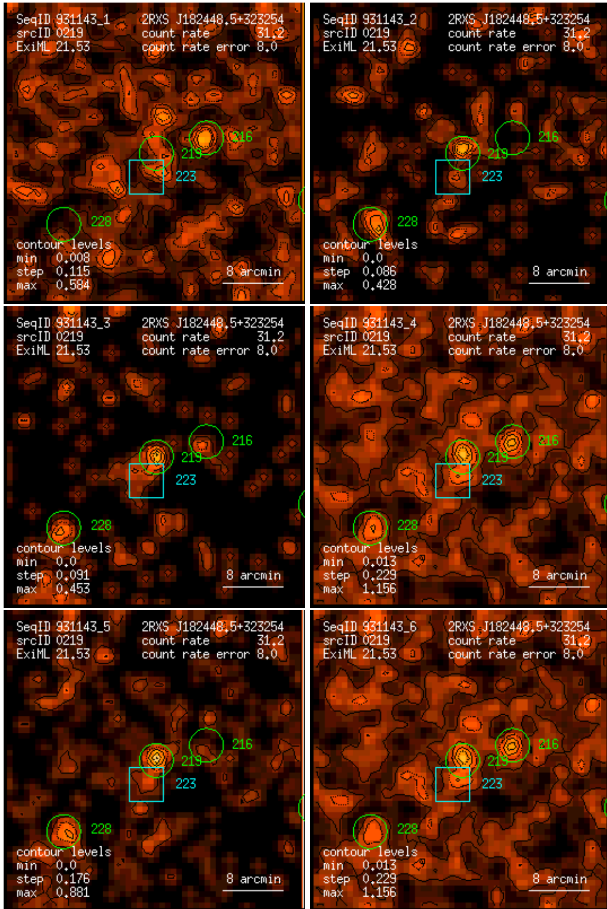
Figure 219: RASS 931143: detection 0219: band rate images, Gaussian filter: (1) PSPC channels 11 – 41, (2) 52 – 90, (3) 91 – 201, (4) 11 – 235, (5) 52 – 201, (6) 11 – 201. Broad band rates in counts/ks. Band rate contour levels in counts/ks/arcmin 2 .
