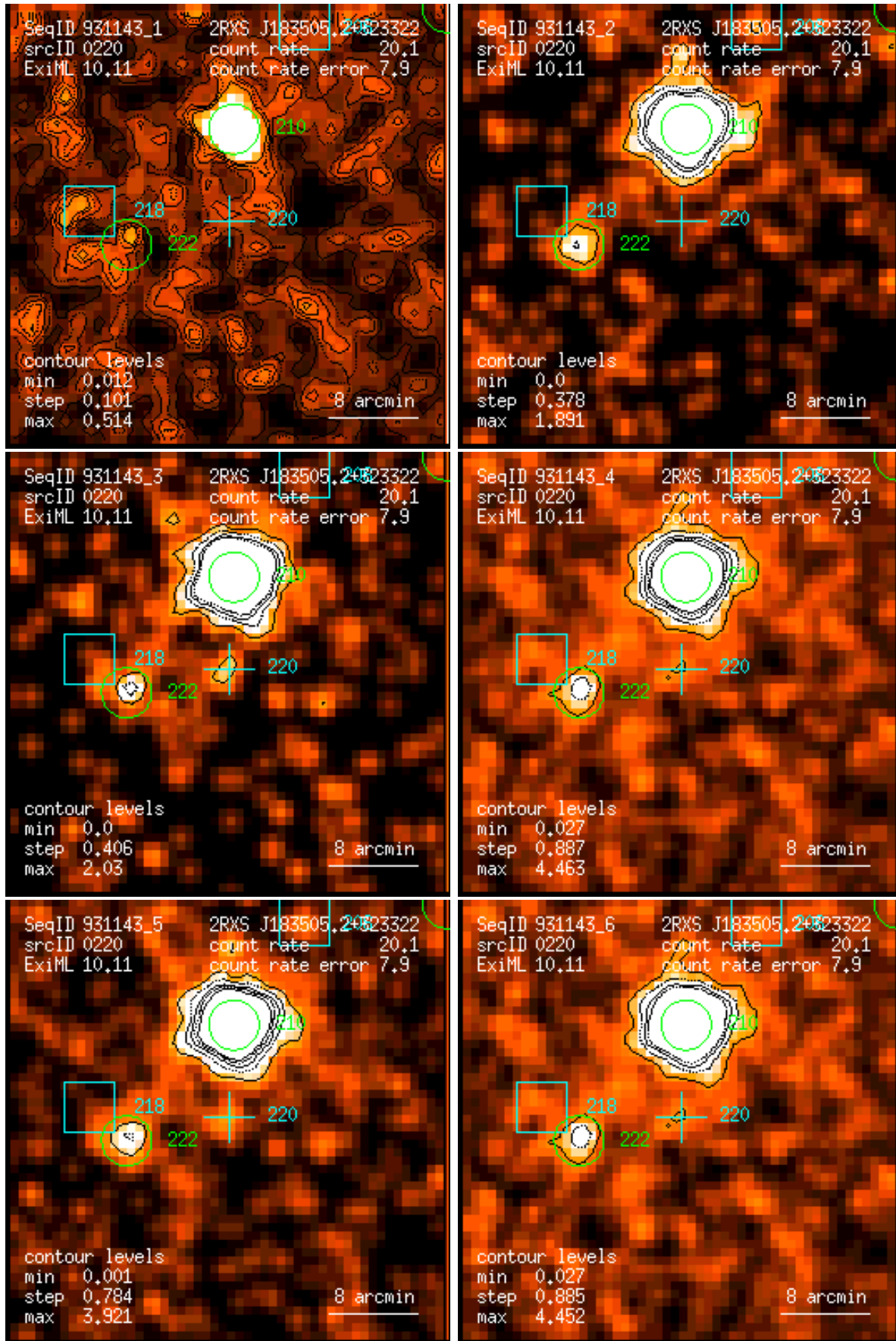
Figure 220: RASS 931143: detection 0220: band rate images, Gaussian filter: (1) PSPC channels 11 – 41, (2) 52 – 90, (3) 91 – 201, (4) 11 – 235, (5) 52 – 201, (6) 11 – 201. Broad band rates in counts/ks. Band rate contour levels in counts/ks/arcmin 2 .
