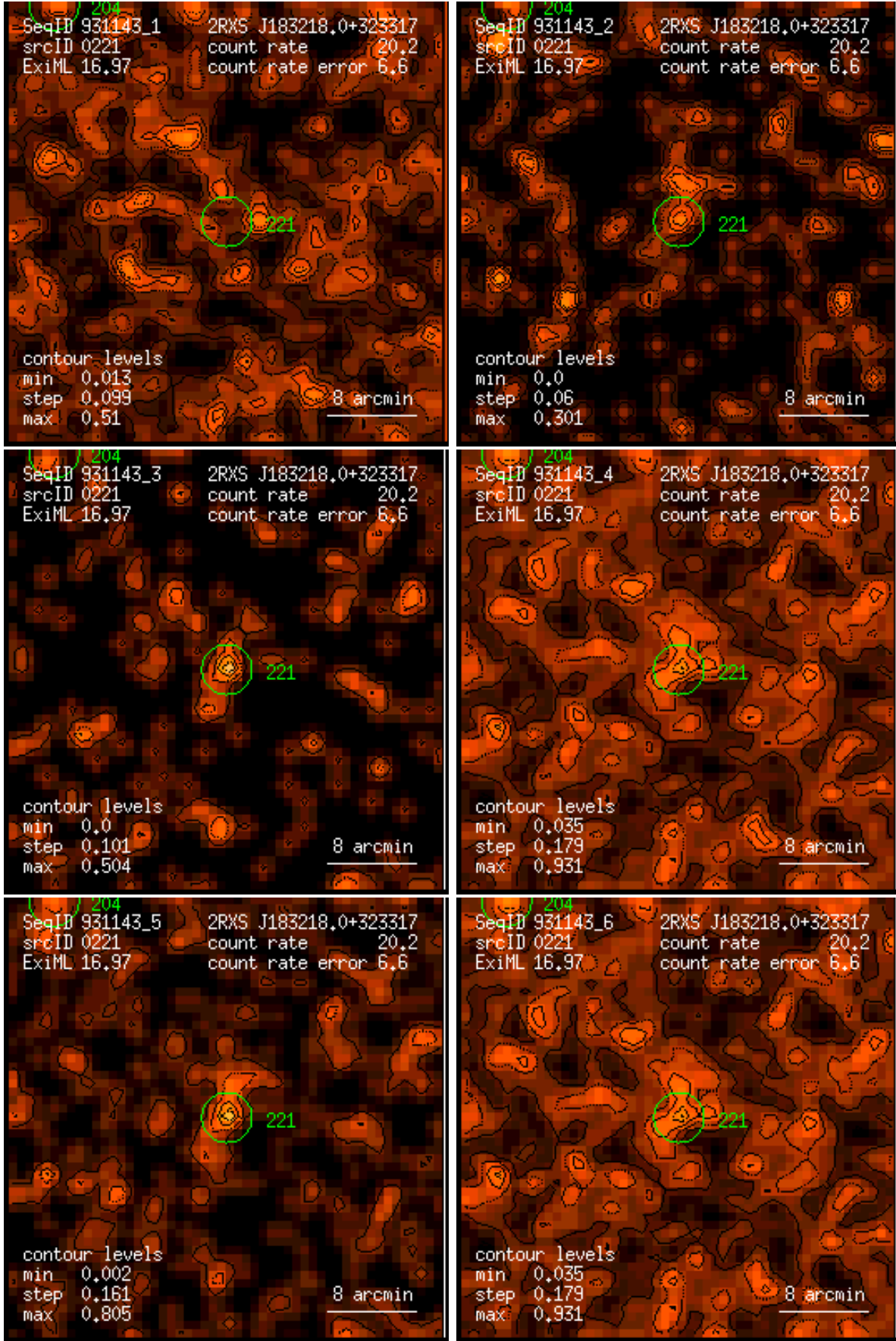
Figure 221: RASS 931143: detection 0221: band rate images, Gaussian filter: (1) PSPC channels 11 – 41, (2) 52 – 90, (3) 91 – 201, (4) 11 – 235, (5) 52 – 201, (6) 11 – 201. Broad band rates in counts/ks. Band rate contour levels in counts/ks/arcmin 2 .
