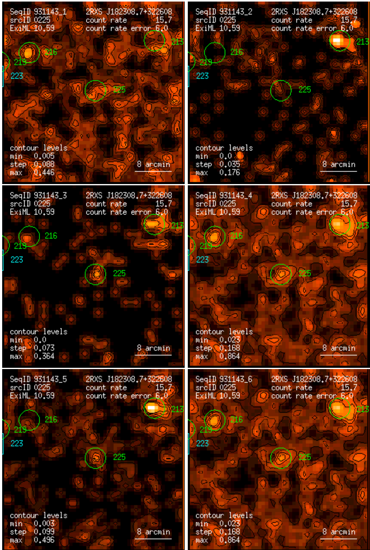
Figure 225: RASS 931143: detection 0225: band rate images, Gaussian filter: (1) PSPC channels 11 – 41, (2) 52 – 90, (3) 91 – 201, (4) 11 – 235, (5) 52 – 201, (6) 11 – 201. Broad band rates in counts/ks. Band rate contour levels in counts/ks/arcmin 2 .
