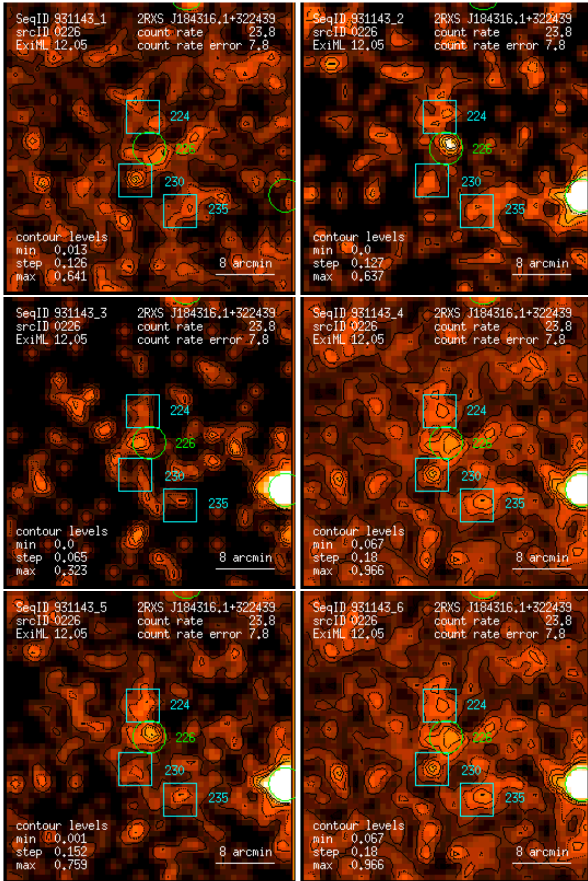
Figure 226: RASS 931143: detection 0226: band rate images, Gaussian filter: (1) PSPC channels 11 – 41, (2) 52 – 90, (3) 91 – 201, (4) 11 – 235, (5) 52 – 201, (6) 11 – 201. Broad band rates in counts/ks. Band rate contour levels in counts/ks/arcmin 2 .
