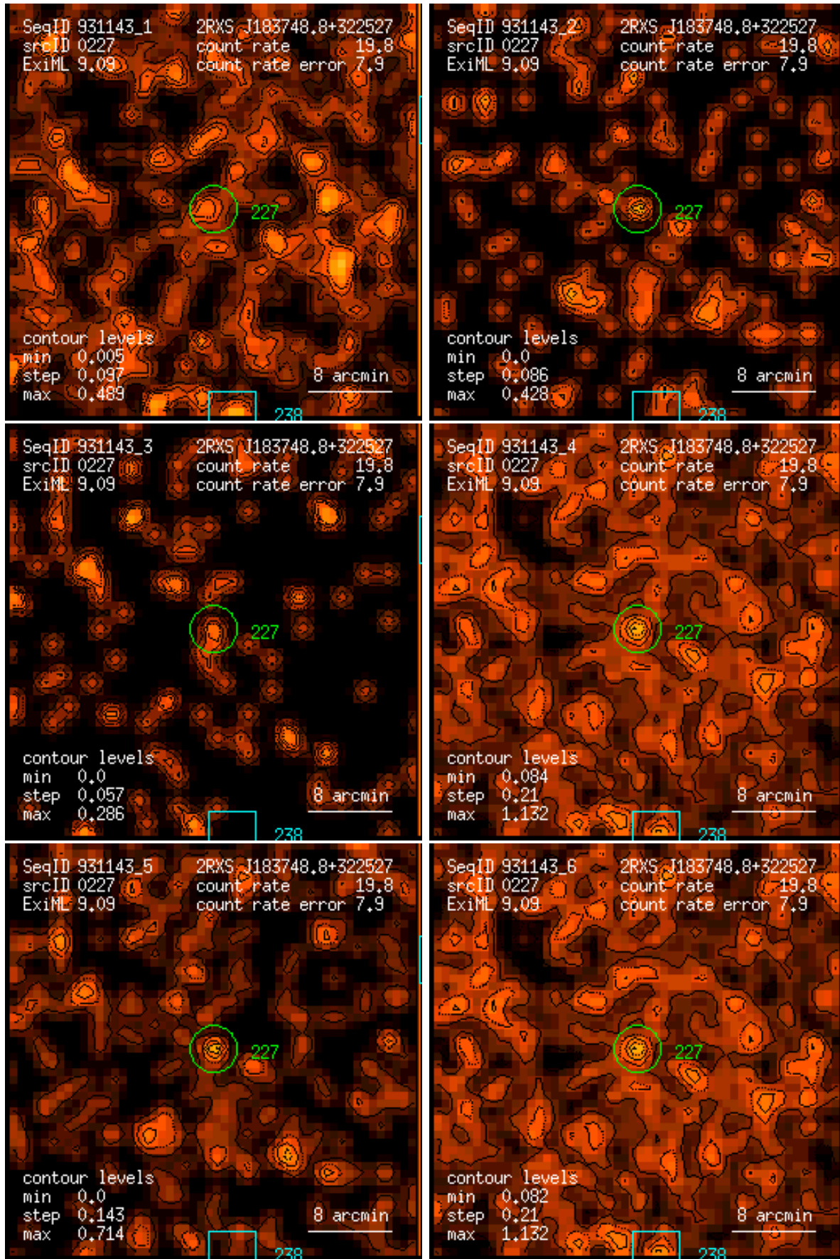
Figure 227: RASS 931143: detection 0227: band rate images, Gaussian filter: (1) PSPC channels 11 – 41, (2) 52 – 90, (3) 91 – 201, (4) 11 – 235, (5) 52 – 201, (6) 11 – 201. Broad band rates in counts/ks. Band rate contour levels in counts/ks/arcmin 2 .
