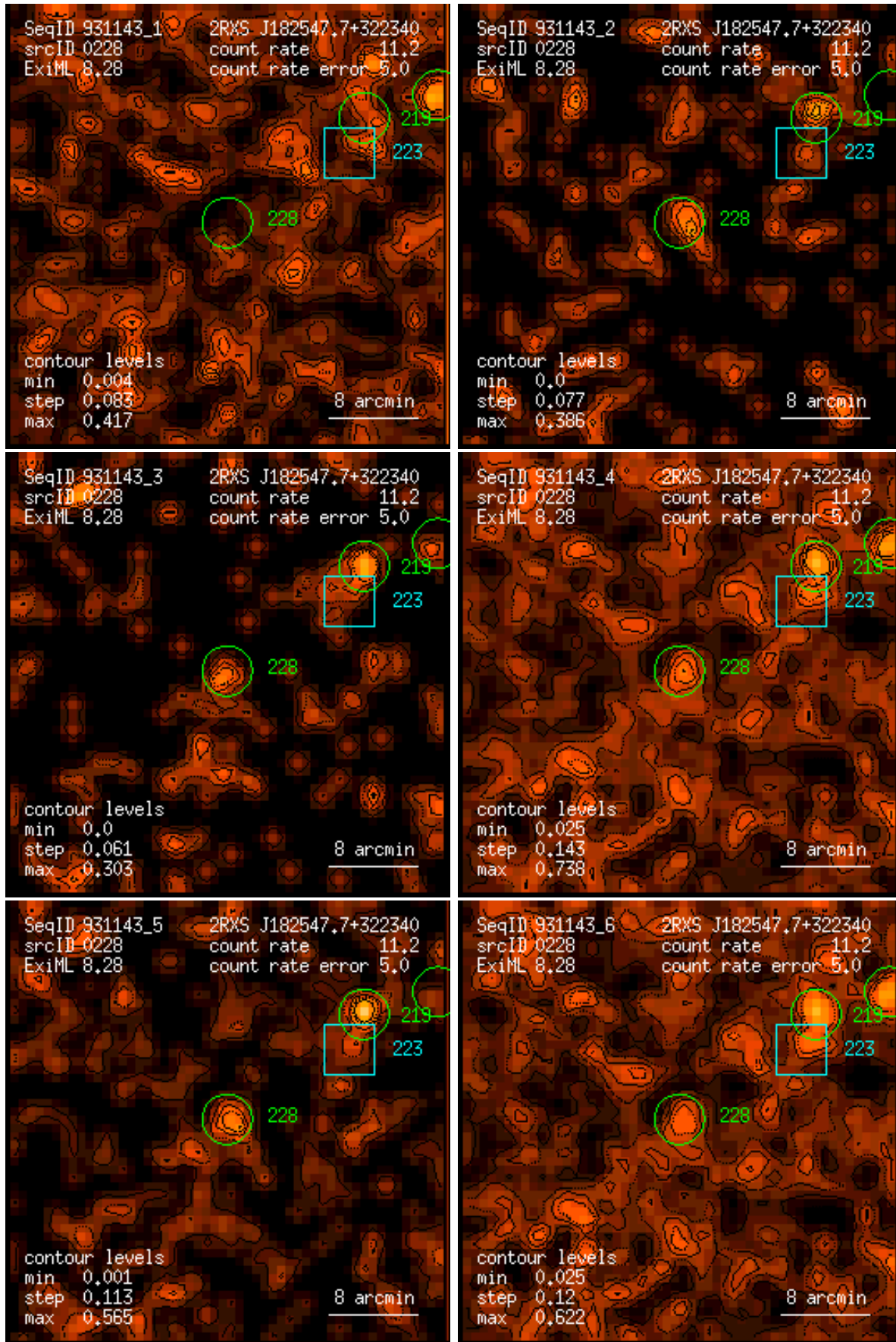
Figure 228: RASS 931143: detection 0228: band rate images, Gaussian filter: (1) PSPC channels 11 – 41, (2) 52 – 90, (3) 91 – 201, (4) 11 – 235, (5) 52 – 201, (6) 11 – 201. Broad band rates in counts/ks. Band rate contour levels in counts/ks/arcmin 2 .
