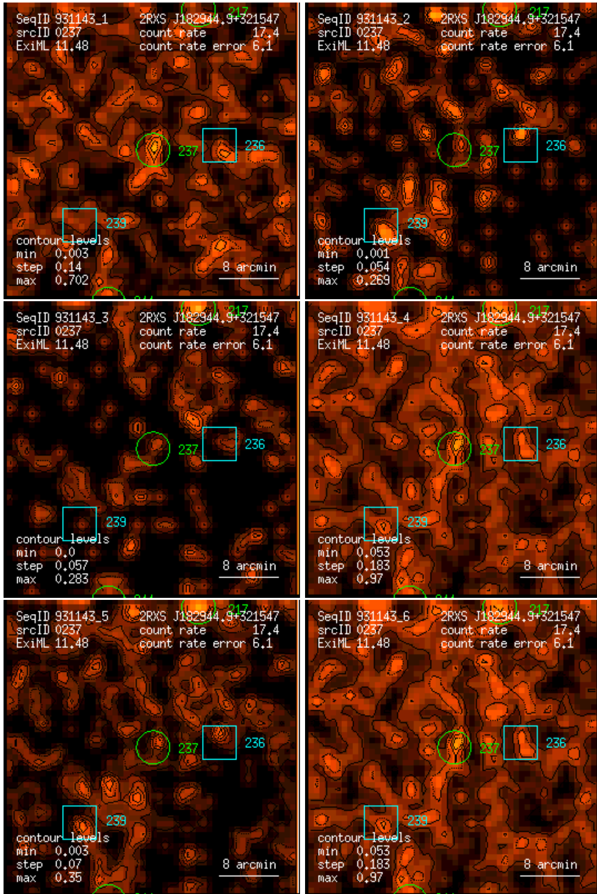
Figure 237: RASS 931143: detection 0237: band rate images, Gaussian filter: (1) PSPC channels 11 – 41, (2) 52 – 90, (3) 91 – 201, (4) 11 – 235, (5) 52 – 201, (6) 11 – 201. Broad band rates in counts/ks. Band rate contour levels in counts/ks/arcmin 2 .
