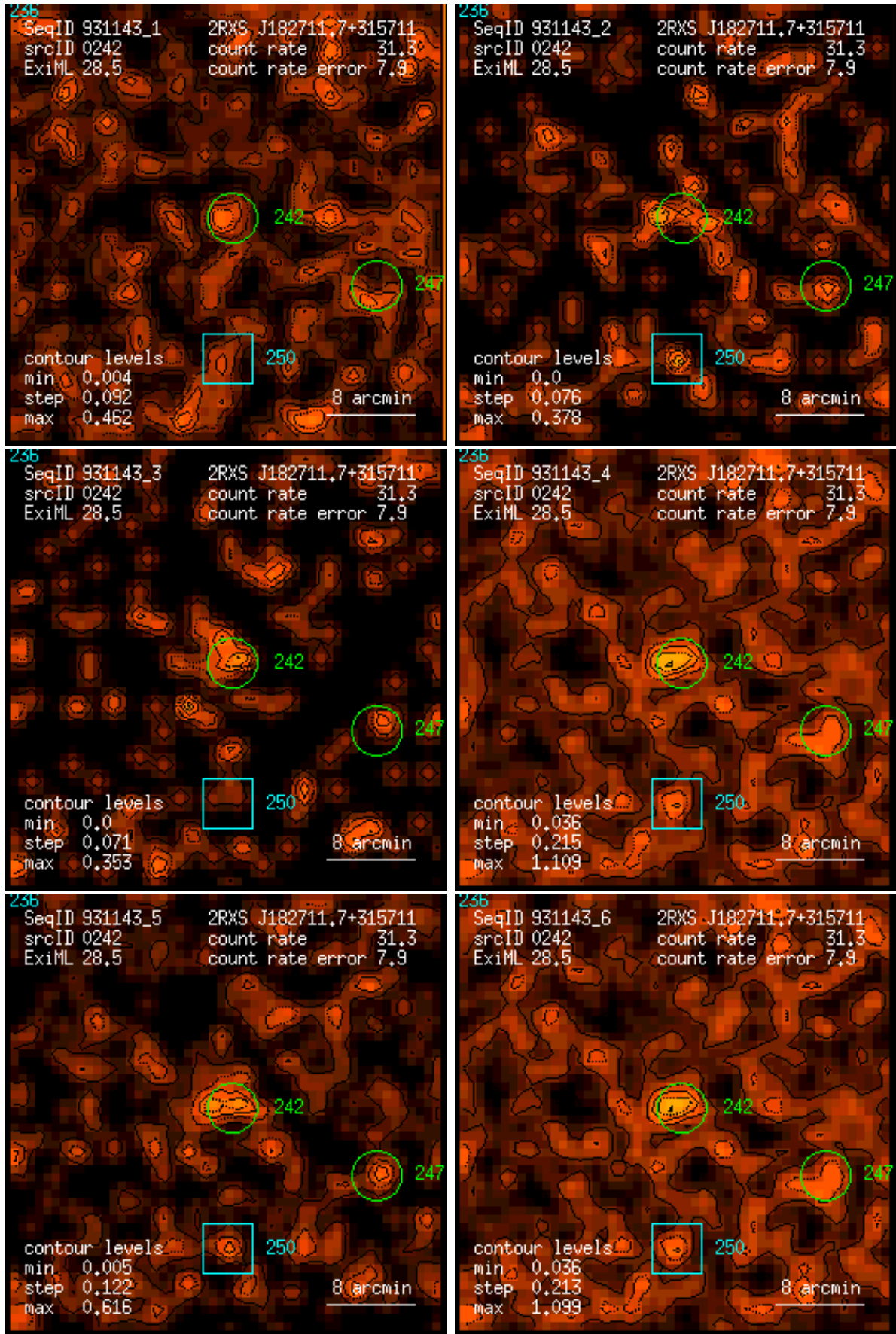
Figure 242: RASS 931143: detection 0242: band rate images, Gaussian filter: (1) PSPC channels 11 – 41, (2) 52 – 90, (3) 91 – 201, (4) 11 – 235, (5) 52 – 201, (6) 11 – 201. Broad band rates in counts/ks. Band rate contour levels in counts/ks/arcmin 2 .
