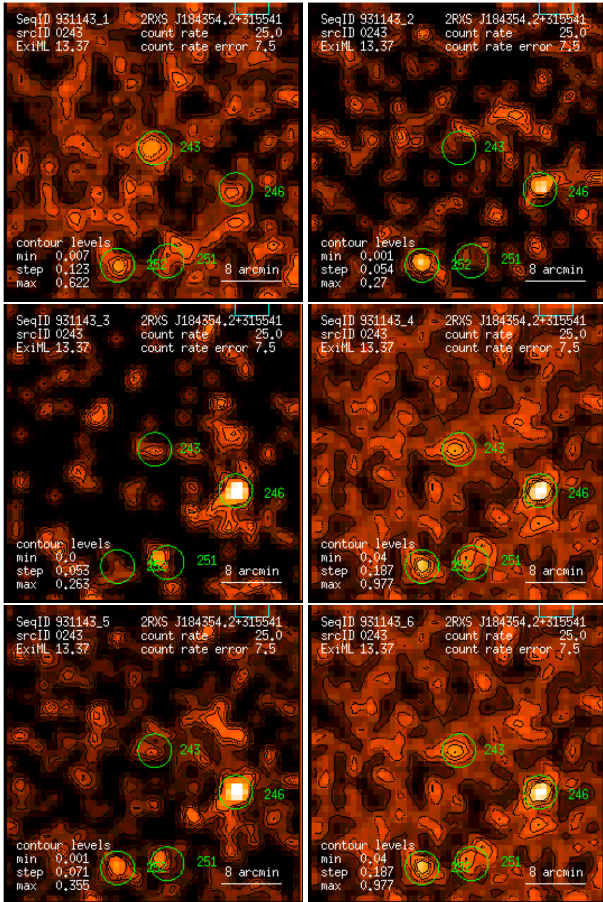
Figure 243: RASS 931143: detection 0243: band rate images, Gaussian filter: (1) PSPC channels 11 – 41, (2) 52 – 90, (3) 91 – 201, (4) 11 – 235, (5) 52 – 201, (6) 11 – 201. Broad band rates in counts/ks. Band rate contour levels in counts/ks/arcmin 2 .
