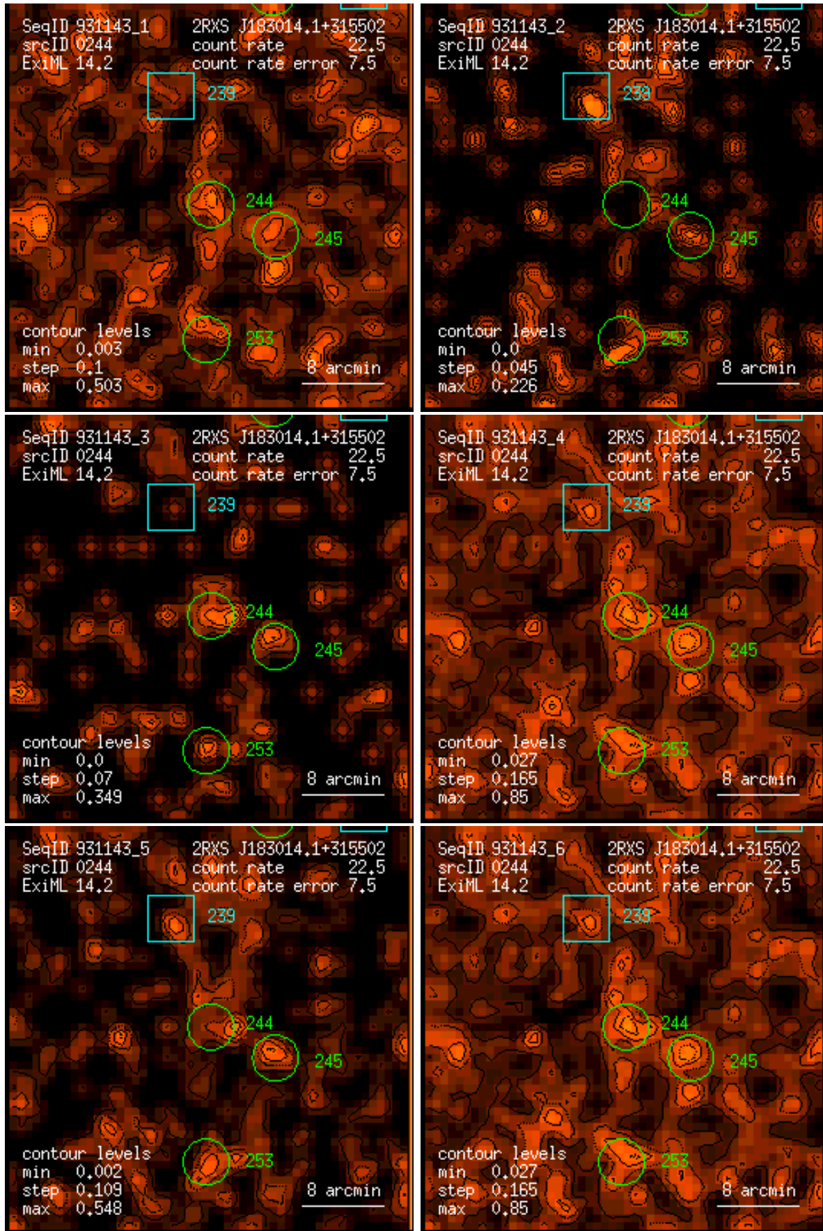
Figure 244: RASS 931143: detection 0244: band rate images, Gaussian filter: (1) PSPC channels 11 – 41, (2) 52 – 90, (3) 91 – 201, (4) 11 – 235, (5) 52 – 201, (6) 11 – 201. Broad band rates in counts/ks. Band rate contour levels in counts/ks/arcmin 2 .
