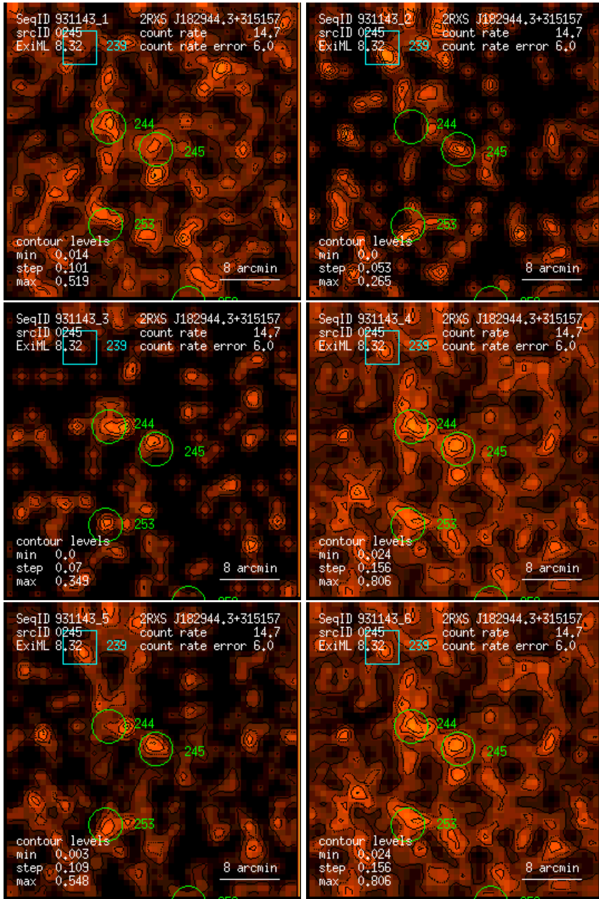
Figure 245: RASS 931143: detection 0245: band rate images, Gaussian filter: (1) PSPC channels 11 – 41, (2) 52 – 90, (3) 91 – 201, (4) 11 – 235, (5) 52 – 201, (6) 11 – 201. Broad band rates in counts/ks. Band rate contour levels in counts/ks/arcmin 2 .
