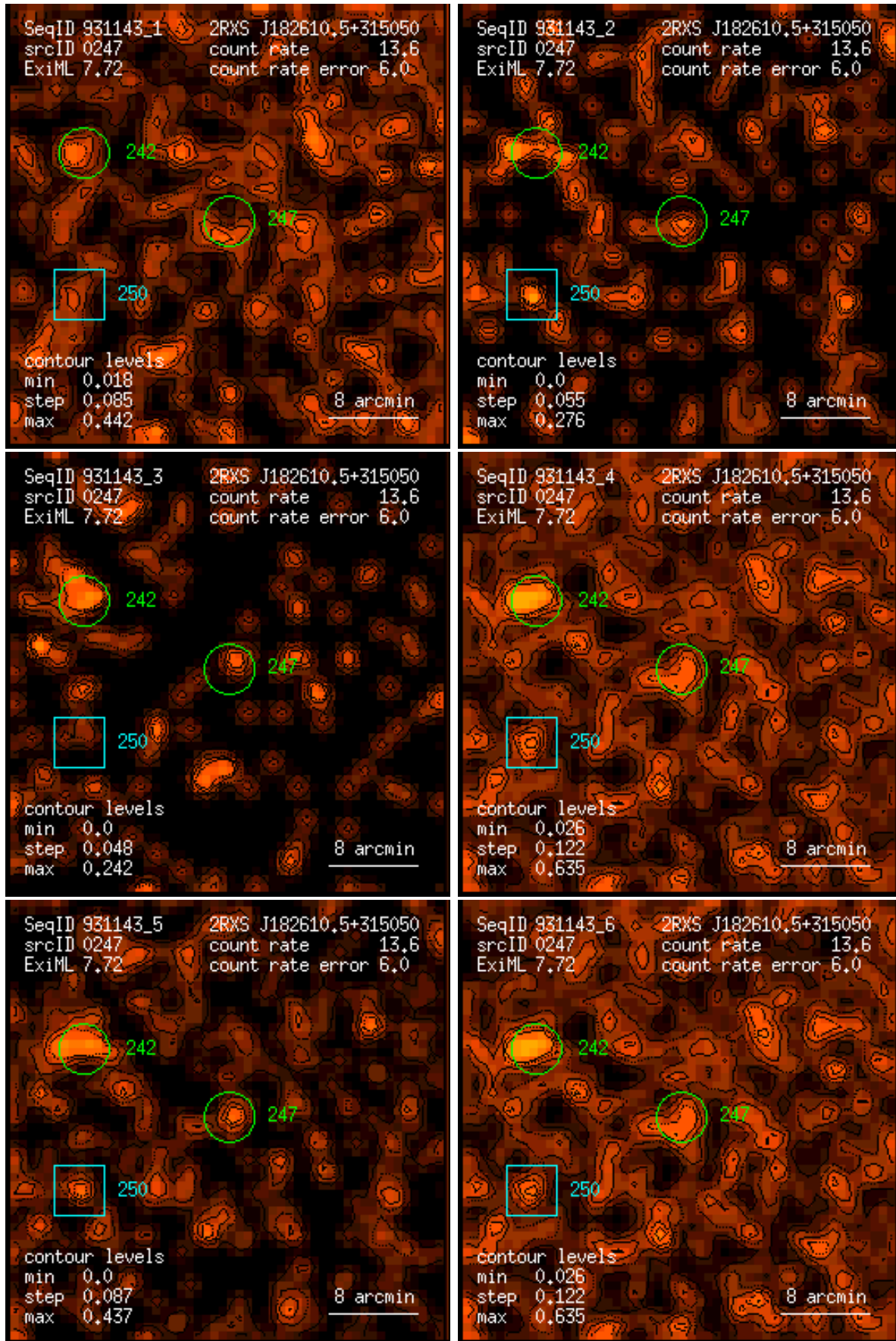
Figure 247: RASS 931143: detection 0247: band rate images, Gaussian filter: (1) PSPC channels 11 – 41, (2) 52 – 90, (3) 91 – 201, (4) 11 – 235, (5) 52 – 201, (6) 11 – 201. Broad band rates in counts/ks. Band rate contour levels in counts/ks/arcmin 2 .
