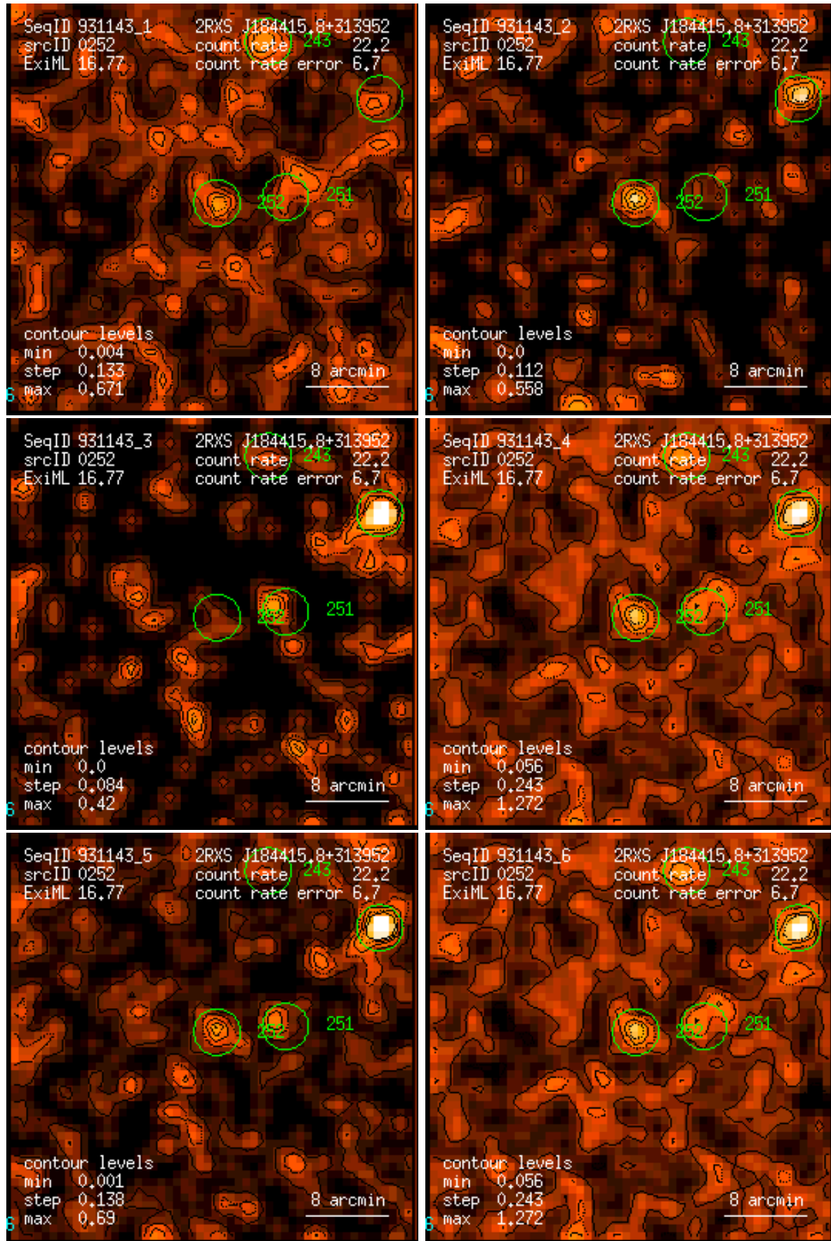
Figure 252: RASS 931143: detection 0252: band rate images, Gaussian filter: (1) PSPC channels 11 – 41, (2) 52 – 90, (3) 91 – 201, (4) 11 – 235, (5) 52 – 201, (6) 11 – 201. Broad band rates in counts/ks. Band rate contour levels in counts/ks/arcmin 2 .
