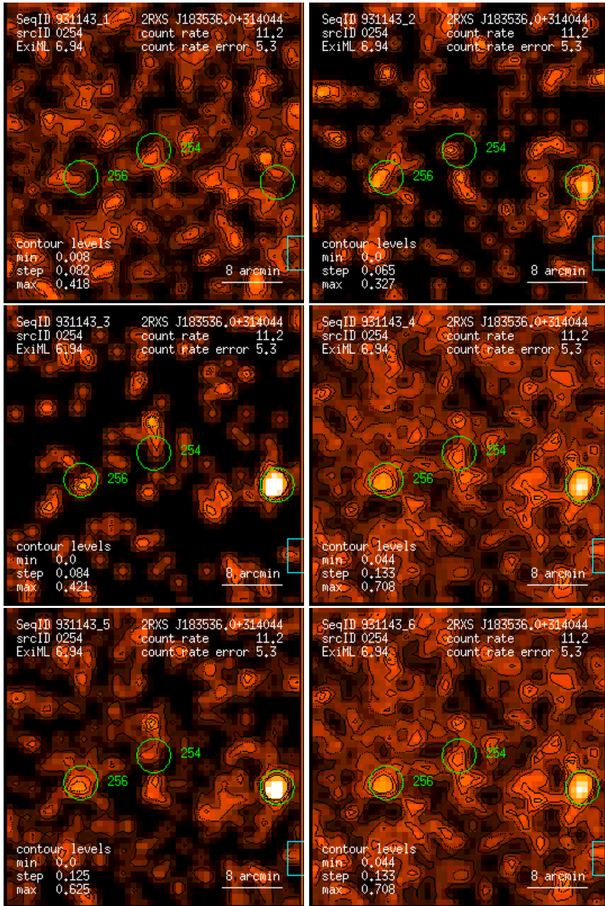
Figure 254: RASS 931143: detection 0254: band rate images, Gaussian filter: (1) PSPC channels 11 – 41, (2) 52 – 90, (3) 91 – 201, (4) 11 – 235, (5) 52 – 201, (6) 11 – 201. Broad band rates in counts/ks. Band rate contour levels in counts/ks/arcmin 2 .
