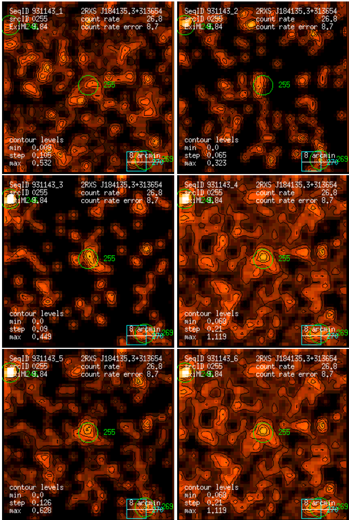
Figure 255: RASS 931143: detection 0255: band rate images, Gaussian filter: (1) PSPC channels 11 – 41, (2) 52 – 90, (3) 91 – 201, (4) 11 – 235, (5) 52 – 201, (6) 11 – 201. Broad band rates in counts/ks. Band rate contour levels in counts/ks/arcmin 2 .
