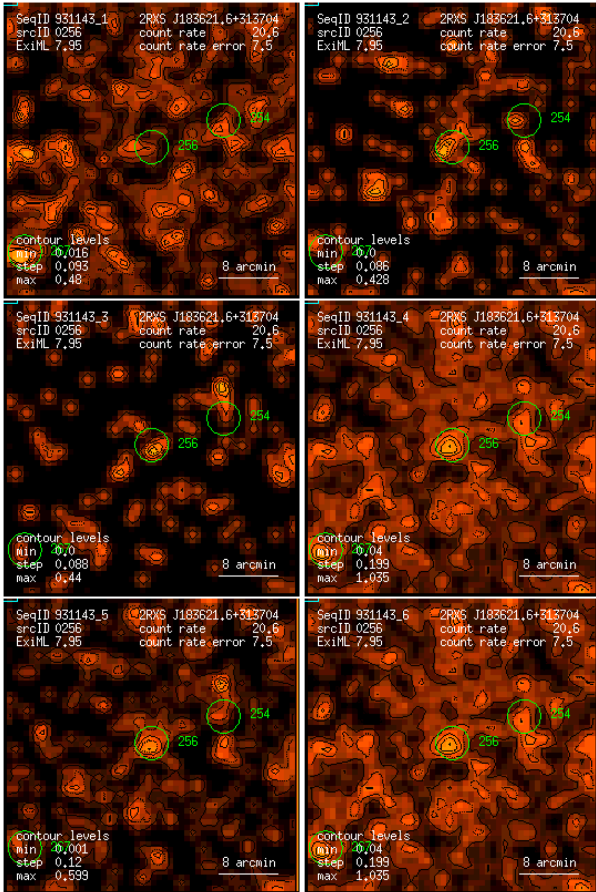
Figure 256: RASS 931143: detection 0256: band rate images, Gaussian filter: (1) PSPC channels 11 – 41, (2) 52 – 90, (3) 91 – 201, (4) 11 – 235, (5) 52 – 201, (6) 11 – 201. Broad band rates in counts/ks. Band rate contour levels in counts/ks/arcmin 2 .
