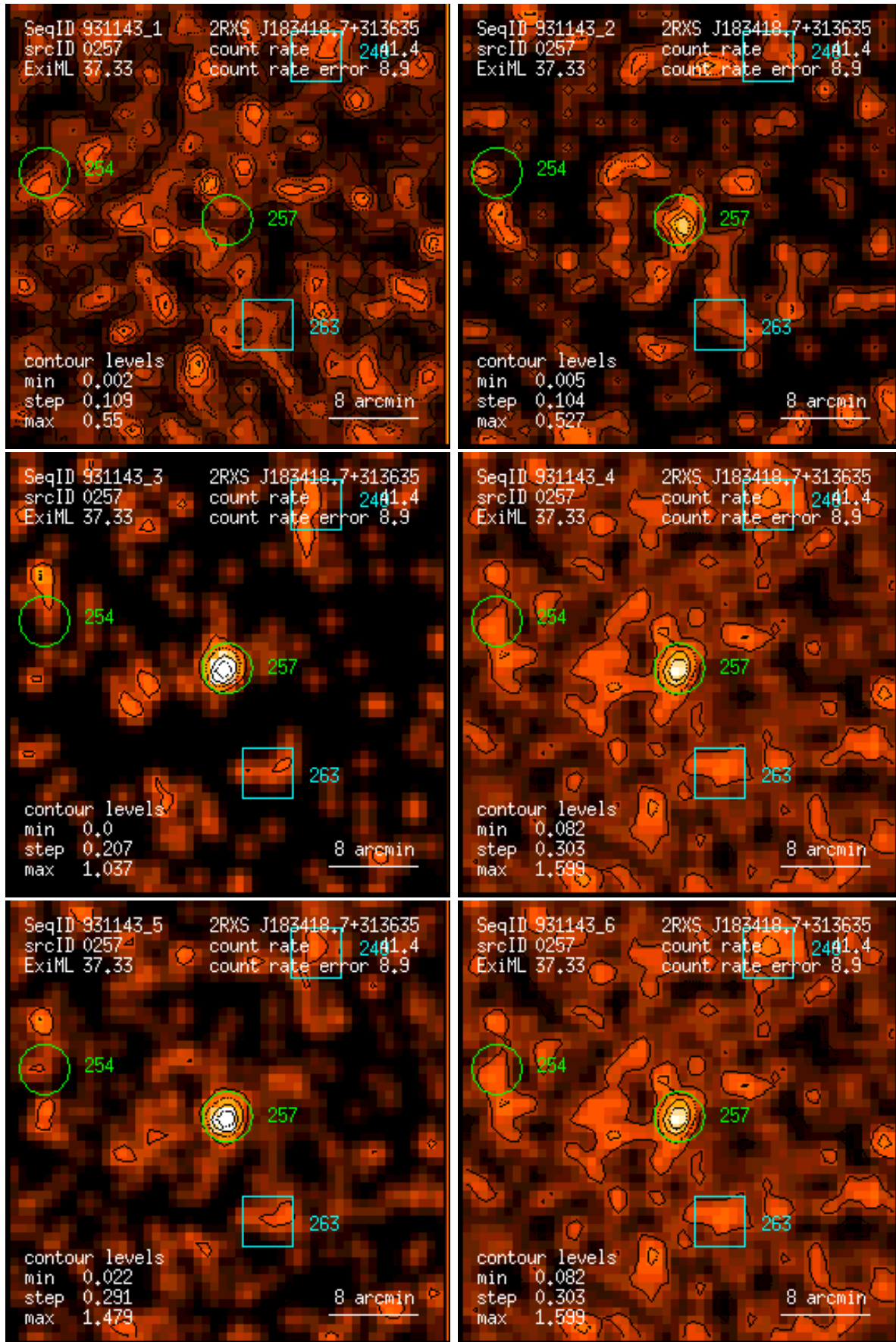
Figure 257: RASS 931143: detection 0257: band rate images, Gaussian filter: (1) PSPC channels 11 – 41, (2) 52 – 90, (3) 91 – 201, (4) 11 – 235, (5) 52 – 201, (6) 11 – 201. Broad band rates in counts/ks. Band rate contour levels in counts/ks/arcmin 2 .
