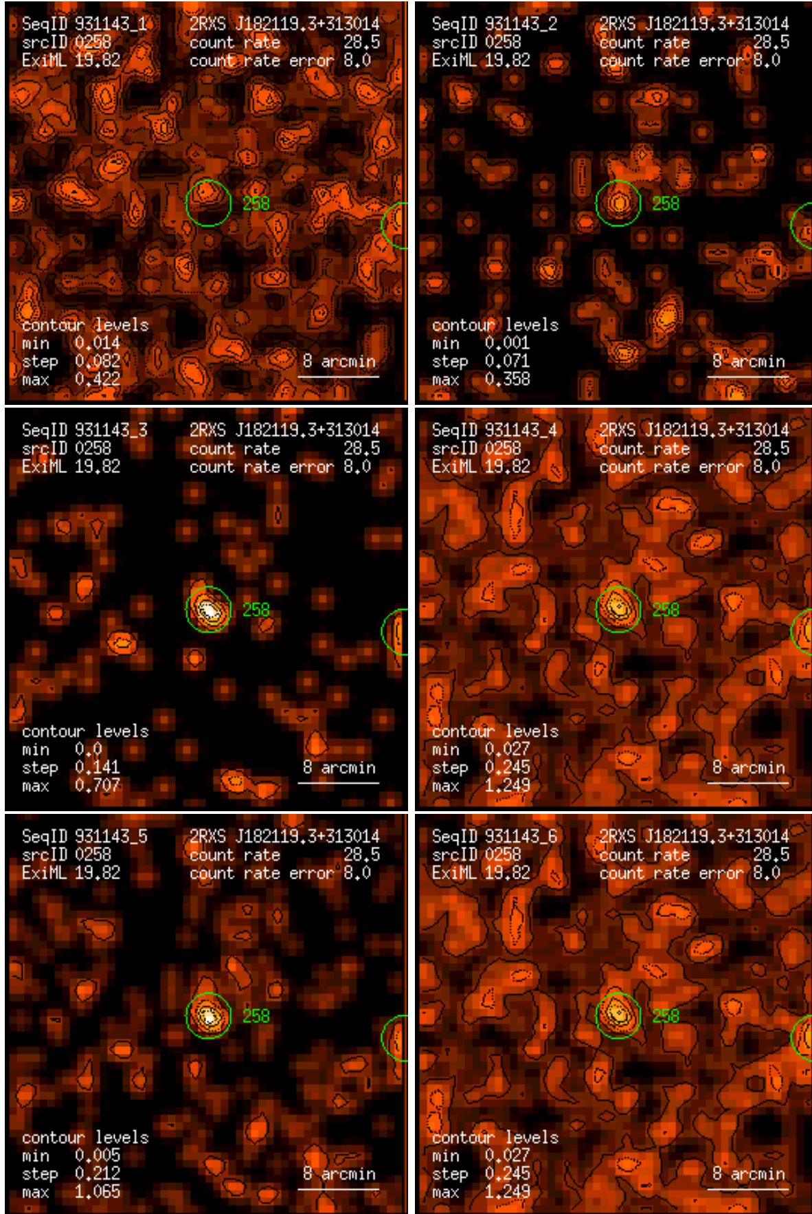
Figure 258: RASS 931143: detection 0258: band rate images, Gaussian filter: (1) PSPC channels 11 – 41, (2) 52 – 90, (3) 91 – 201, (4) 11 – 235, (5) 52 – 201, (6) 11 – 201. Broad band rates in counts/ks. Band rate contour levels in counts/ks/arcmin 2 .
