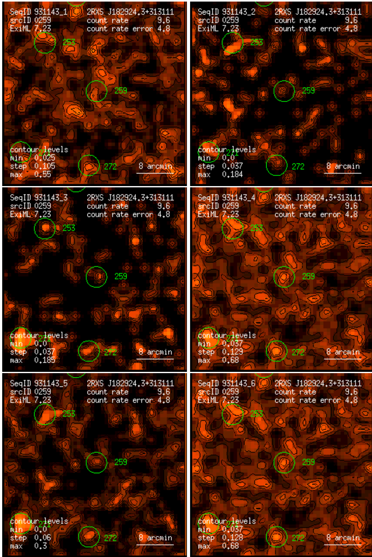
Figure 259: RASS 931143: detection 0259: band rate images, Gaussian filter: (1) PSPC channels 11 – 41, (2) 52 – 90, (3) 91 – 201, (4) 11 – 235, (5) 52 – 201, (6) 11 – 201. Broad band rates in counts/ks. Band rate contour levels in counts/ks/arcmin 2 .
