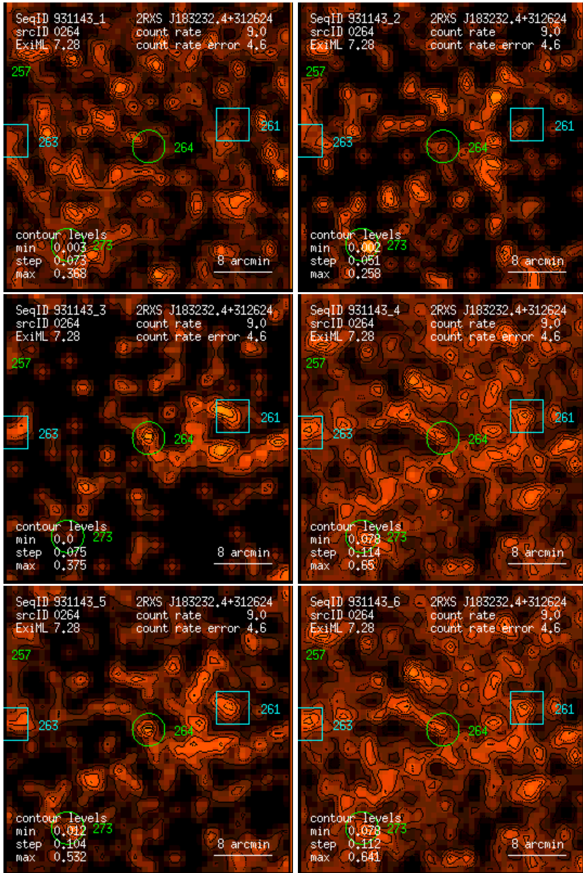
Figure 264: RASS 931143: detection 0264: band rate images, Gaussian filter: (1) PSPC channels 11 – 41, (2) 52 – 90, (3) 91 – 201, (4) 11 – 235, (5) 52 – 201, (6) 11 – 201. Broad band rates in counts/ks. Band rate contour levels in counts/ks/arcmin 2 .
