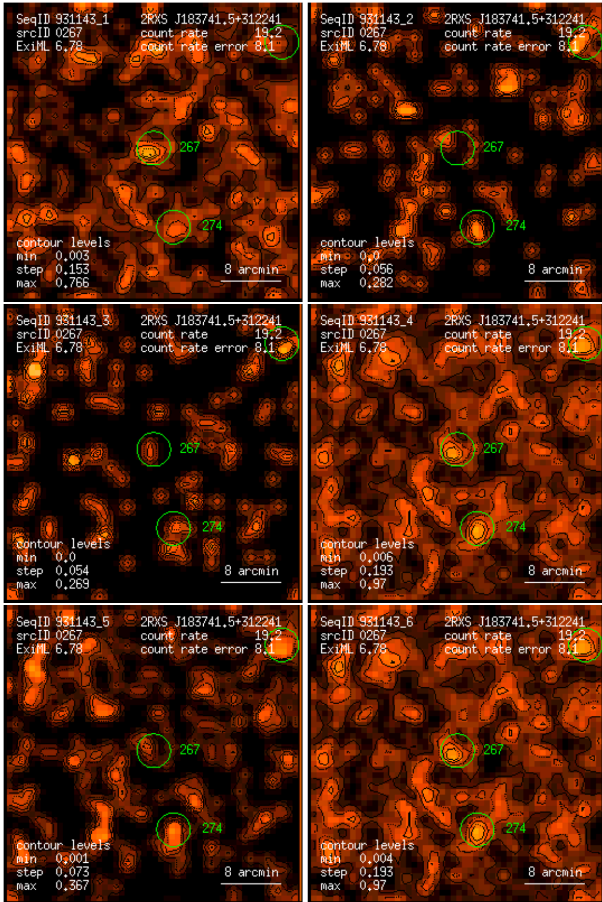
Figure 267: RASS 931143: detection 0267: band rate images, Gaussian filter: (1) PSPC channels 11 – 41, (2) 52 – 90, (3) 91 – 201, (4) 11 – 235, (5) 52 – 201, (6) 11 – 201. Broad band rates in counts/ks. Band rate contour levels in counts/ks/arcmin 2 .
